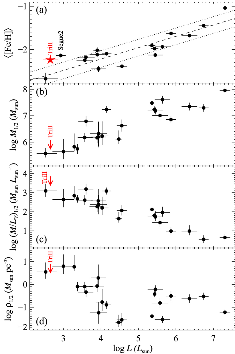
Figure 7. from Triangulum II. Not Especially Dense After All null 2017 APJ 838 83 doi:10.3847/1538-4357/aa6570 https://dx.doi.org/10.3847/1538-4357/aa6570 © 2017. The American Astronomical Society. All rights reserved.
