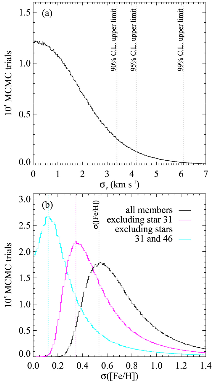
Figure 6. from Triangulum II. Not Especially Dense After All null 2017 APJ 838 83 doi:10.3847/1538-4357/aa6570 https://dx.doi.org/10.3847/1538-4357/aa6570 © 2017. The American Astronomical Society. All rights reserved.
