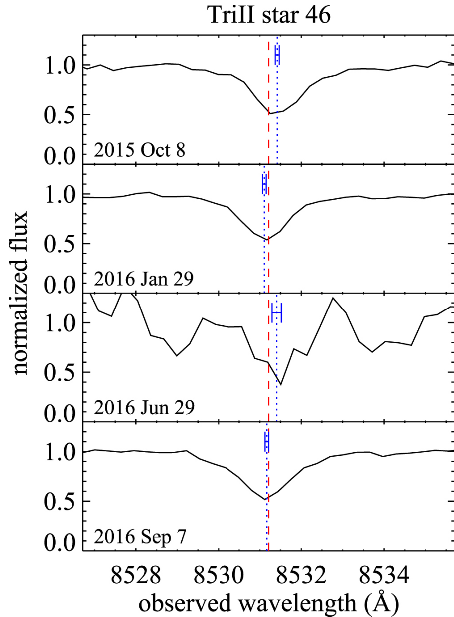
Figure 5. from Triangulum II. Not Especially Dense After All null 2017 APJ 838 83 doi:10.3847/1538-4357/aa6570 https://dx.doi.org/10.3847/1538-4357/aa6570 © 2017. The American Astronomical Society. All rights reserved.
