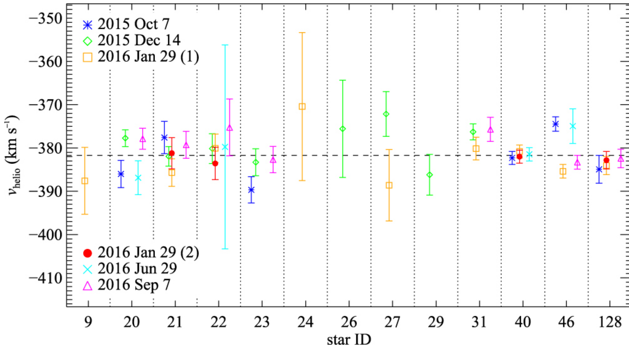
Figure 4. from Triangulum II. Not Especially Dense After All null 2017 APJ 838 83 doi:10.3847/1538-4357/aa6570 https://dx.doi.org/10.3847/1538-4357/aa6570 © 2017. The American Astronomical Society. All rights reserved.
