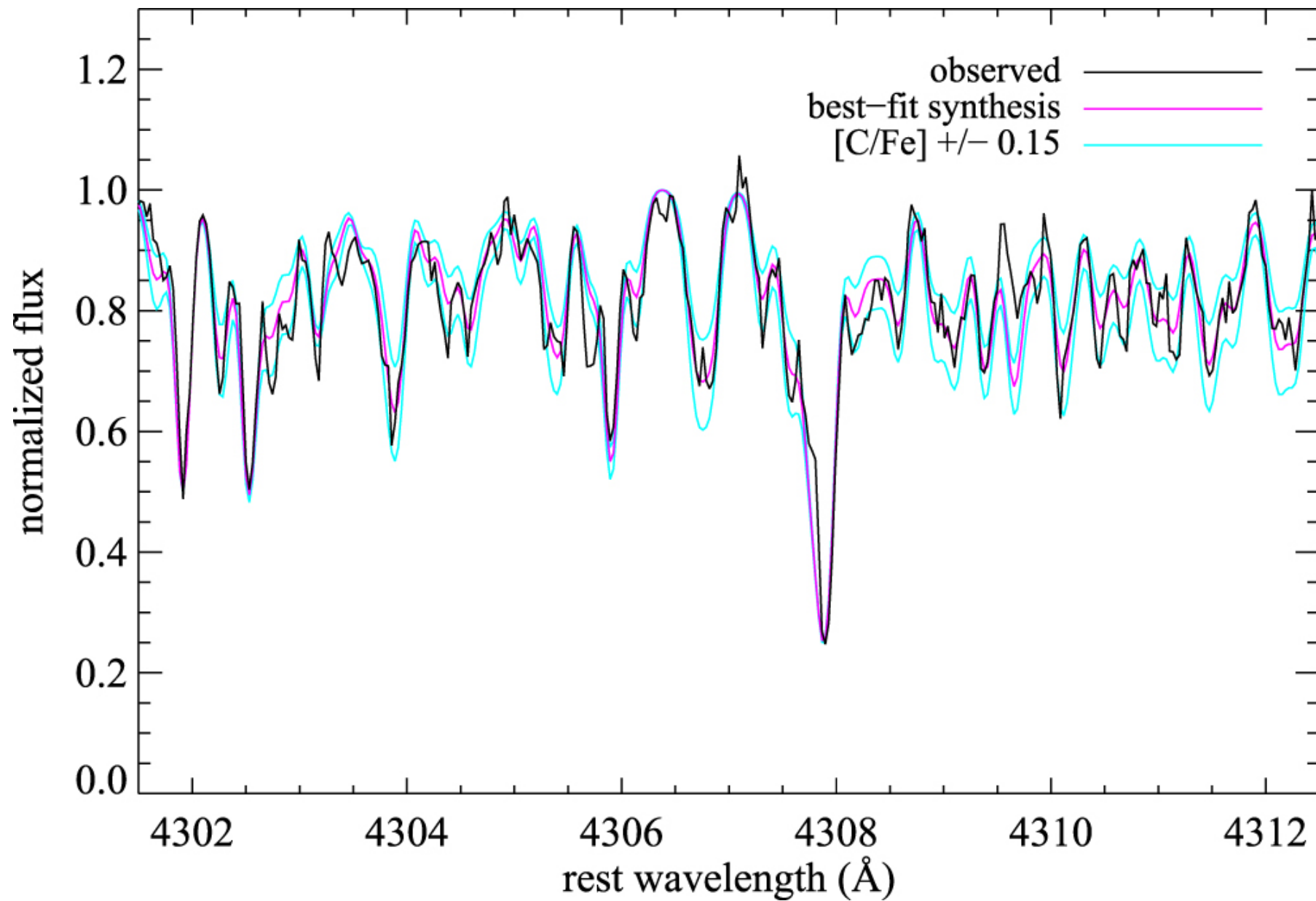
Figure 10. from Triangulum II. Not Especially Dense After All null 2017 APJ 838 83 doi:10.3847/1538-4357/aa6570 https://dx.doi.org/10.3847/1538-4357/aa6570 © 2017. The American Astronomical Society. All rights reserved.
