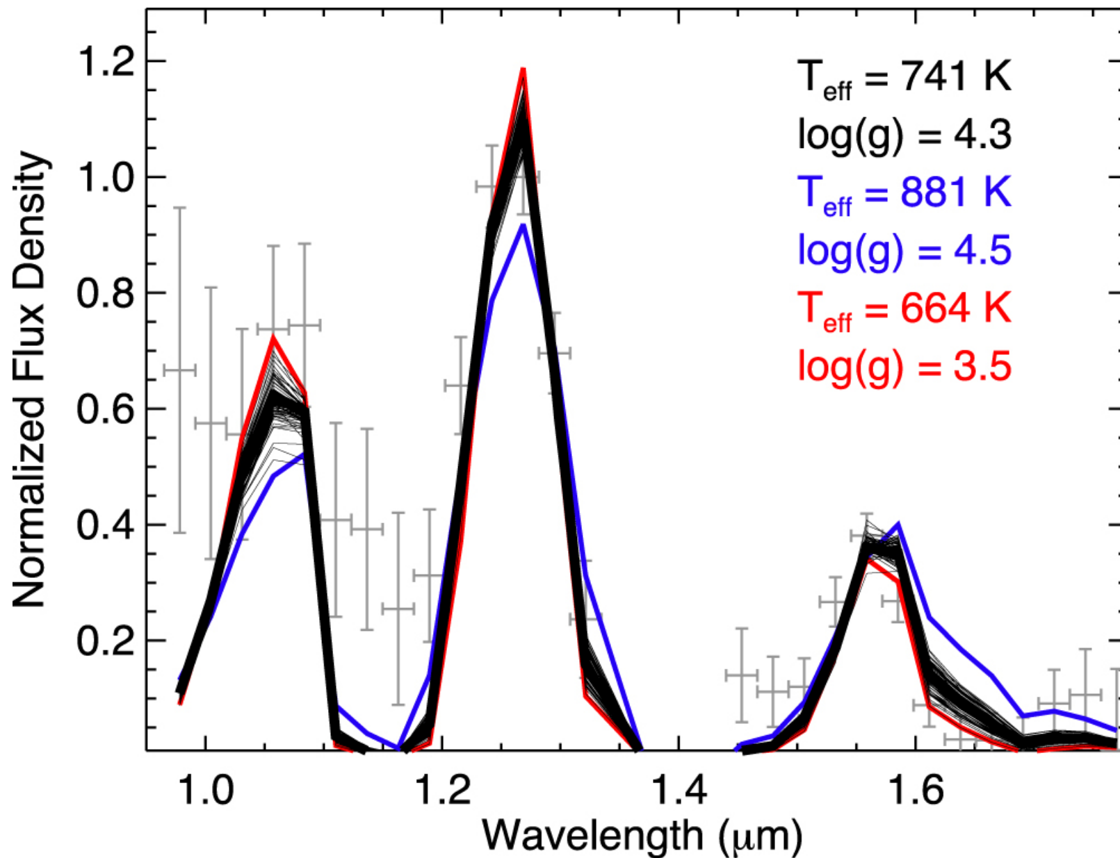
Figure 8. from Project 1640 Observations of Brown Dwarf GJ 758 B: Near-infrared Spectrum and Atmospheric Modeling null 2017 APJ 838 64 doi:10.3847/1538-4357/aa643c https://dx.doi.org/10.3847/1538-4357/aa643c © 2017. The American Astronomical Society. All rights reserved.
