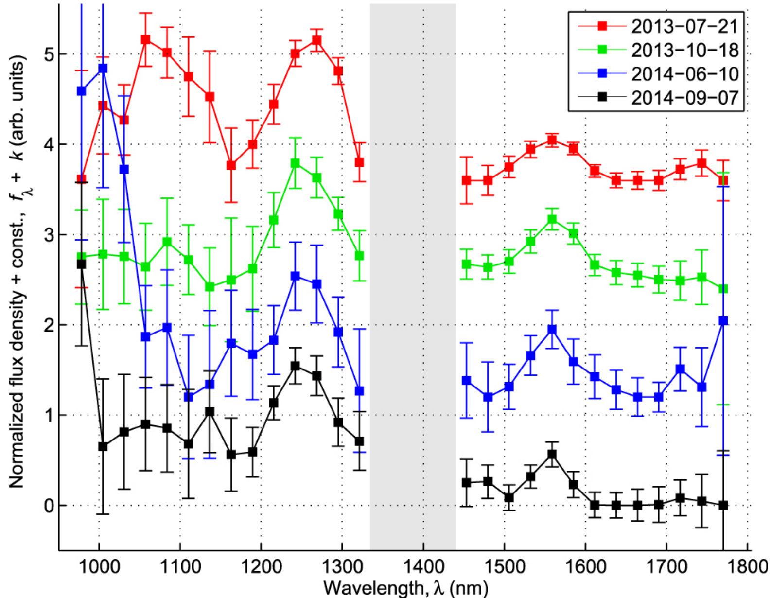
Figure 5. from Project 1640 Observations of Brown Dwarf GJ 758 B: Near-infrared Spectrum and Atmospheric Modeling null 2017 APJ 838 64 doi:10.3847/1538-4357/aa643c https://dx.doi.org/10.3847/1538-4357/aa643c © 2017. The American Astronomical Society. All rights reserved.
