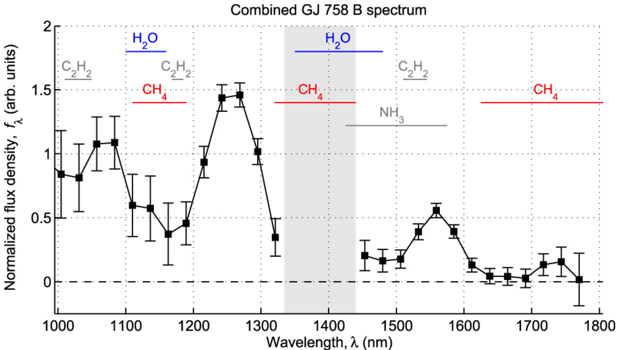
Figure 11. from Project 1640 Observations of Brown Dwarf GJ 758 B: Near-infrared Spectrum and Atmospheric Modeling null 2017 APJ 838 64 doi:10.3847/1538-4357/aa643c https://dx.doi.org/10.3847/1538-4357/aa643c © 2017. The American Astronomical Society. All rights reserved.
