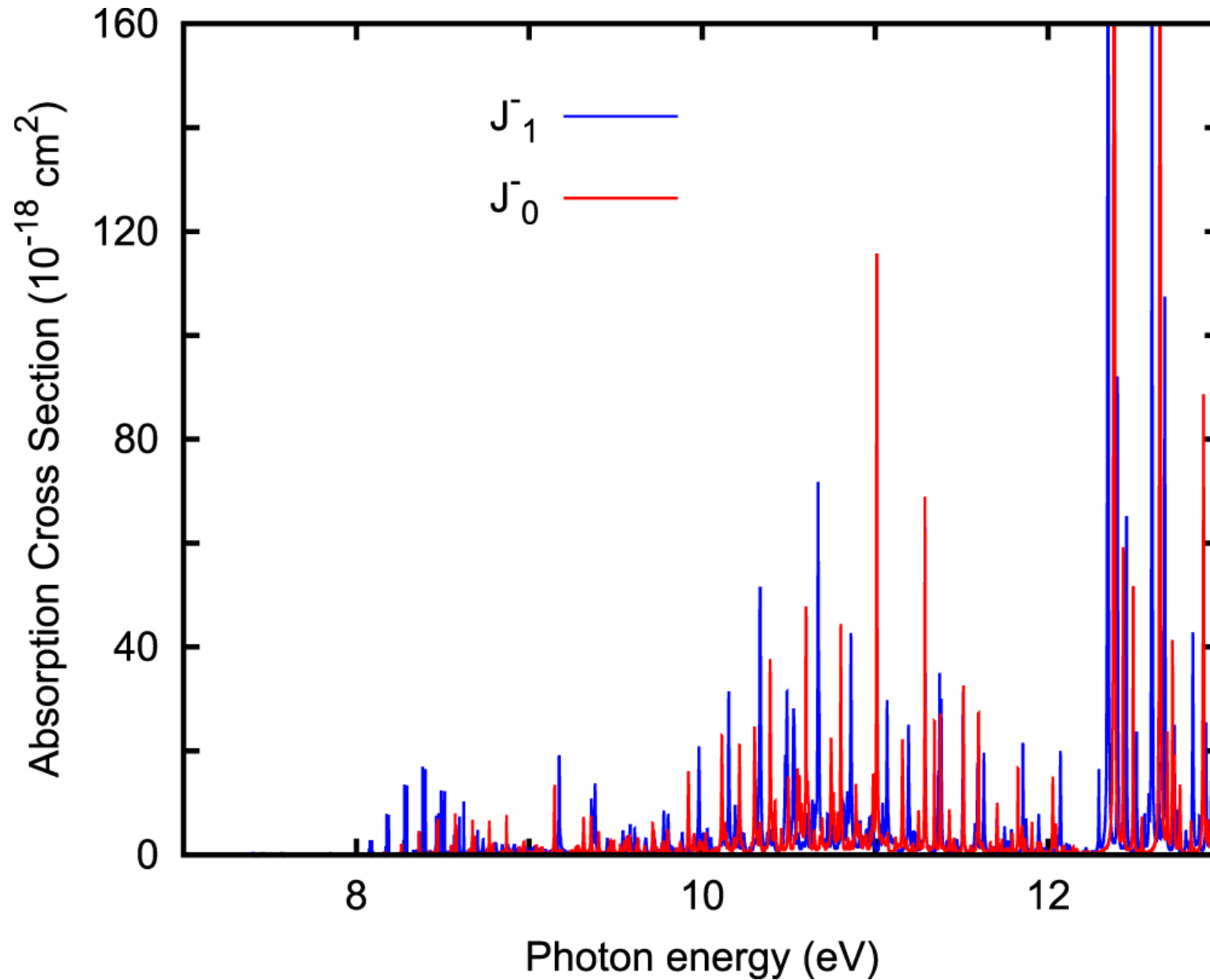
Figure 7. from The Photodissociation of HCN and HNC: Effects on the HNC/HCN Abundance Ratio in the Interstellar Medium null 2017 APJ 838 33 doi:10.3847/1538-4357/aa63ee https://dx.doi.org/10.3847/1538-4357/aa63ee © 2017. The American Astronomical Society. All rights reserved.
