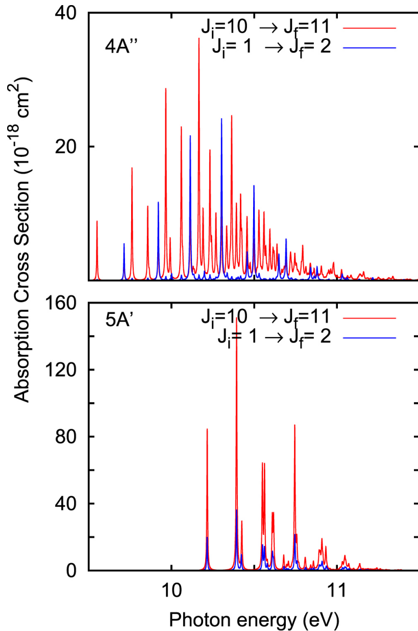
Figure 6. from The Photodissociation of HCN and HNC: Effects on the HNC/HCN Abundance Ratio in the Interstellar Medium null 2017 APJ 838 33 doi:10.3847/1538-4357/aa63ee https://dx.doi.org/10.3847/1538-4357/aa63ee © 2017. The American Astronomical Society. All rights reserved.
