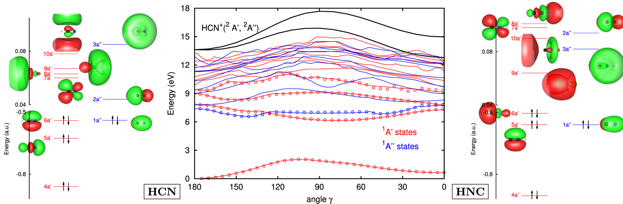
Figure 1. from The Photodissociation of HCN and HNC: Effects on the HNC/HCN Abundance Ratio in the Interstellar Medium null 2017 APJ 838 33 doi:10.3847/1538-4357/aa63ee https://dx.doi.org/10.3847/1538-4357/aa63ee © 2017. The American Astronomical Society. All rights reserved.
