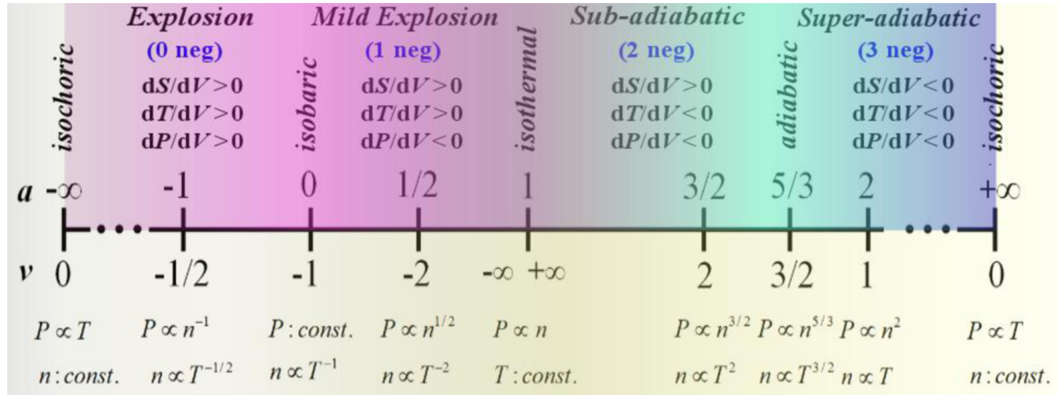
Figure 5. from Modeling the Plasma Flow in the Inner Heliosheath with a Spatially Varying Compression Ratio null 2017 APJ 838 7 doi:10.3847/1538-4357/aa61ff https://dx.doi.org/10.3847/1538-4357/aa61ff © 2017. The American Astronomical Society. All rights reserved.
