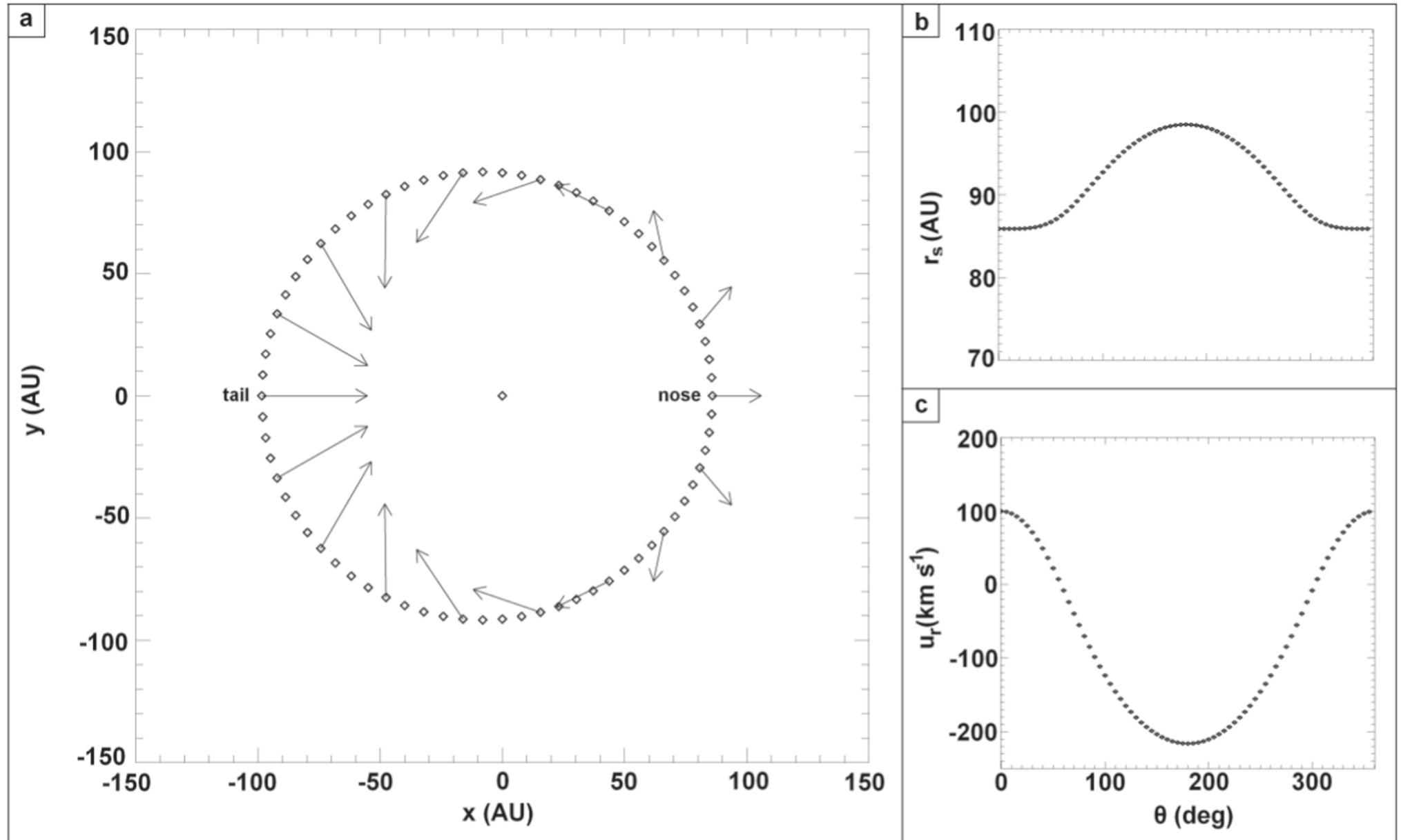
Figure 2. from Modeling the Plasma Flow in the Inner Heliosheath with a Spatially Varying Compression Ratio null 2017 APJ 838 7 doi:10.3847/1538-4357/aa61ff https://dx.doi.org/10.3847/1538-4357/aa61ff © 2017. The American Astronomical Society. All rights reserved.
