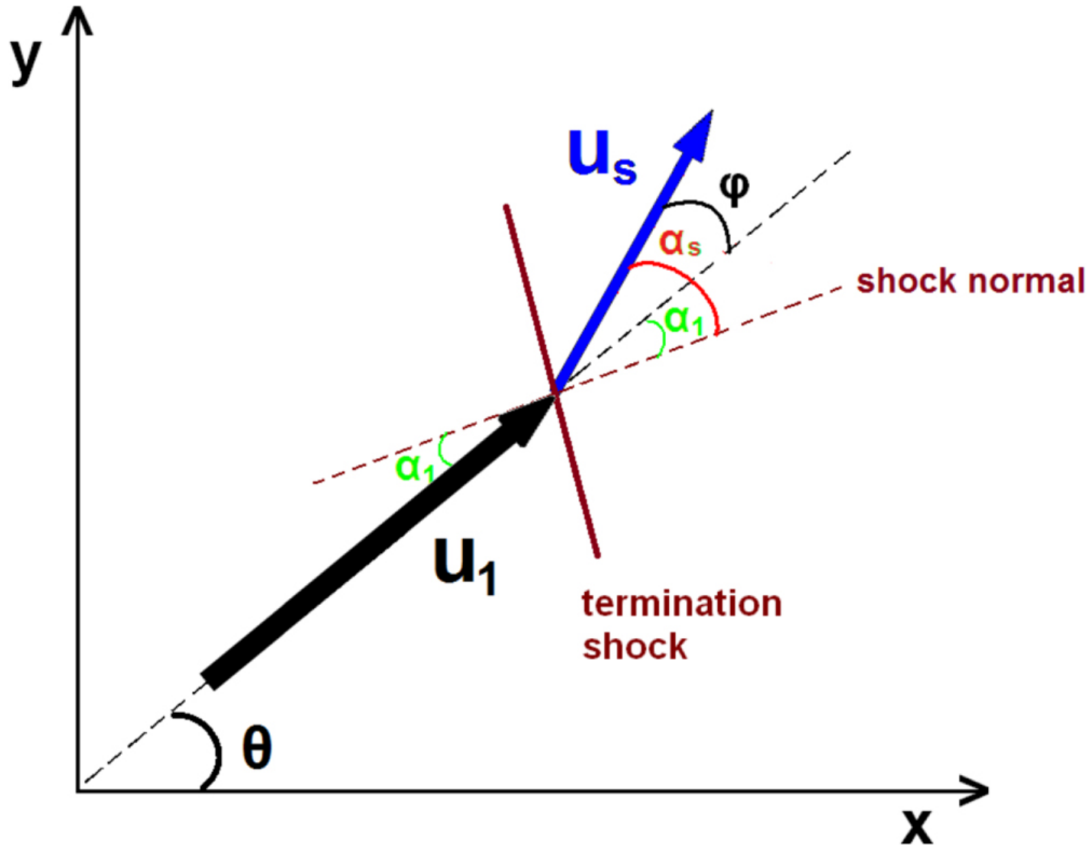
Figure 1. from Modeling the Plasma Flow in the Inner Heliosheath with a Spatially Varying Compression Ratio null 2017 APJ 838 7 doi:10.3847/1538-4357/aa61ff https://dx.doi.org/10.3847/1538-4357/aa61ff © 2017. The American Astronomical Society. All rights reserved.
