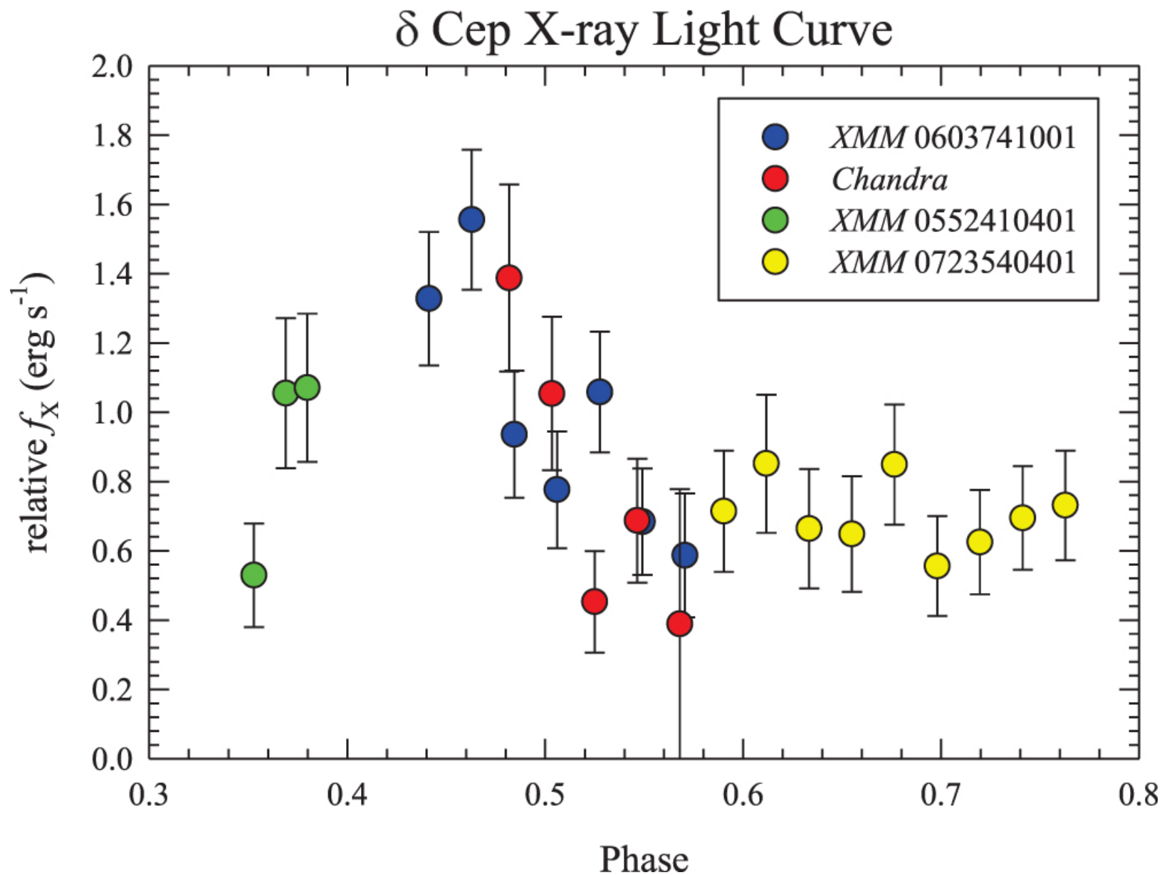
Figure 3. from The Secret Lives of Cepheids: Cep—The Prototype of a New Class of Pulsating X-Ray Variable Stars null 2017 APJ 838 67 doi:10.3847/1538-4357/aa6159 https://dx.doi.org/10.3847/1538-4357/aa6159 © 2017. The American Astronomical Society. All rights reserved.
