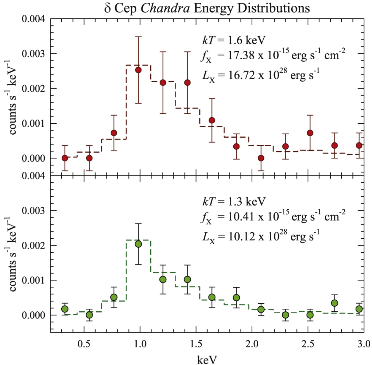
Figure 2. from The Secret Lives of Cepheids: Cep—The Prototype of a New Class of Pulsating X-Ray Variable Stars null 2017 APJ 838 67 doi:10.3847/1538-4357/aa6159 https://dx.doi.org/10.3847/1538-4357/aa6159 © 2017. The American Astronomical Society. All rights reserved.
