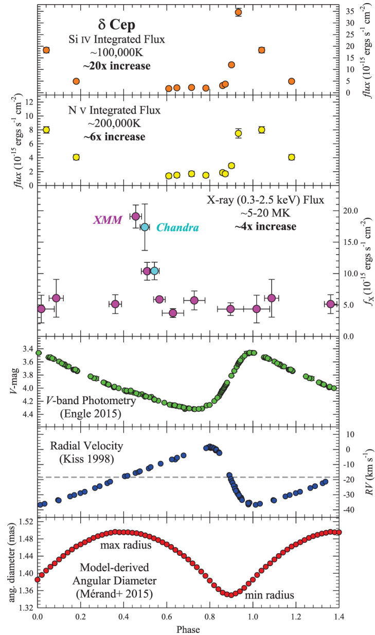
Figure 1. from The Secret Lives of Cepheids: Cep—The Prototype of a New Class of Pulsating X-Ray Variable Stars null 2017 APJ 838 67 doi:10.3847/1538-4357/aa6159 https://dx.doi.org/10.3847/1538-4357/aa6159 © 2017. The American Astronomical Society. All rights reserved.
