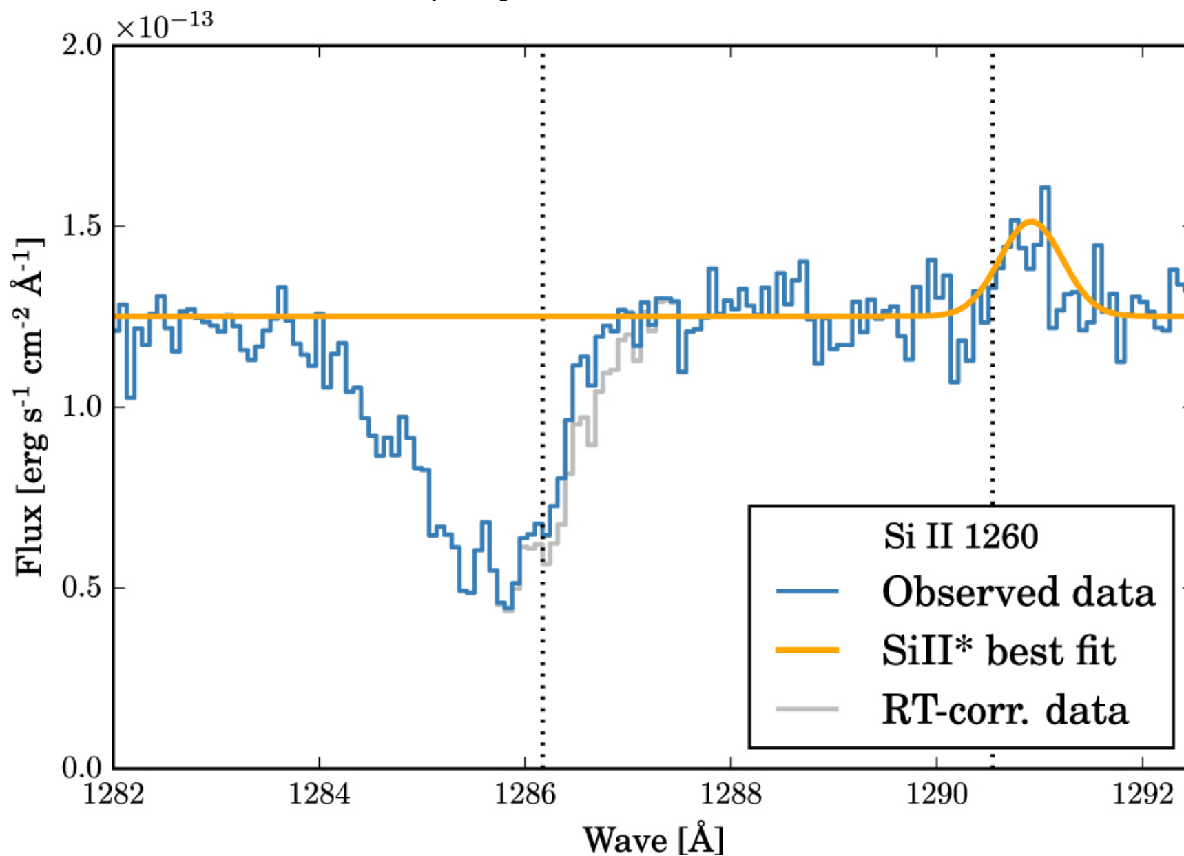
Figure 8. from Neutral ISM, Ly, and Lyman-continuum in the Nearby Starburst Haro 11 null 2017 APJ 837 29 doi:10.3847/1538-4357/aa5d0a https://dx.doi.org/10.3847/1538-4357/aa5d0a © 2017. The American Astronomical Society. All rights reserved.
