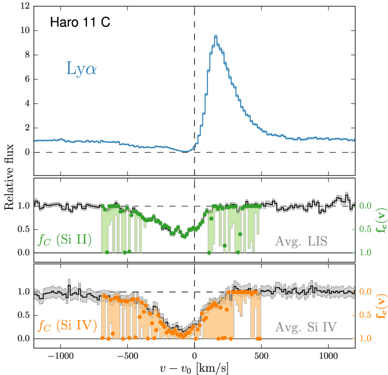
Figure 7. from Neutral ISM, Ly, and Lyman-continuum in the Nearby Starburst Haro 11 null 2017 APJ 837 29 doi:10.3847/1538-4357/aa5d0a https://dx.doi.org/10.3847/1538-4357/aa5d0a © 2017. The American Astronomical Society. All rights reserved.
