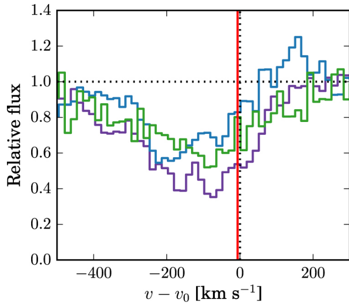
Figure 5. from Neutral ISM, Ly, and Lyman-continuum in the Nearby Starburst Haro 11 null 2017 APJ 837 29 doi:10.3847/1538-4357/aa5d0a https://dx.doi.org/10.3847/1538-4357/aa5d0a © 2017. The American Astronomical Society. All rights reserved.
