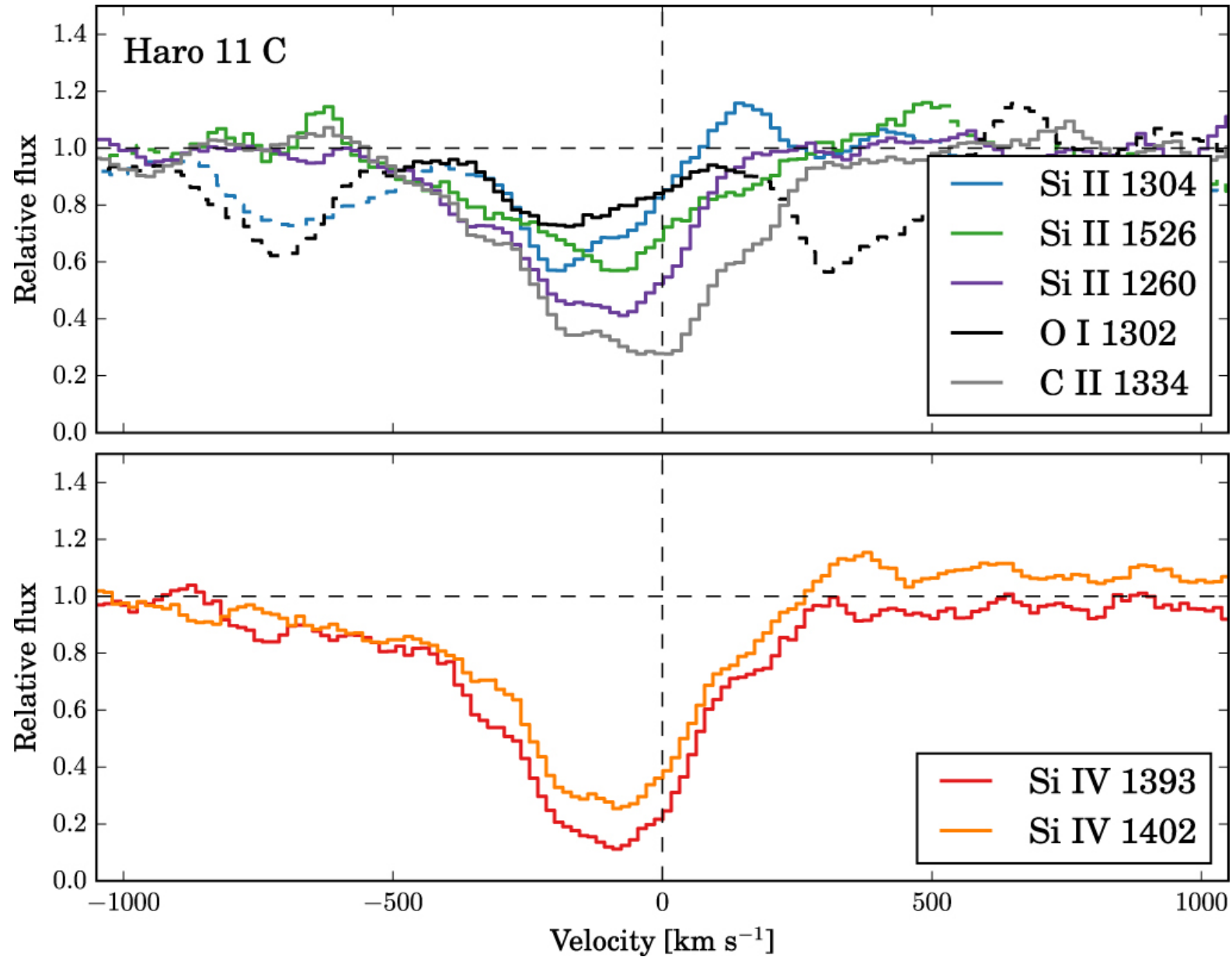
Figure 4. from Neutral ISM, Ly, and Lyman-continuum in the Nearby Starburst Haro 11 null 2017 APJ 837 29 doi:10.3847/1538-4357/aa5d0a https://dx.doi.org/10.3847/1538-4357/aa5d0a © 2017. The American Astronomical Society. All rights reserved.
