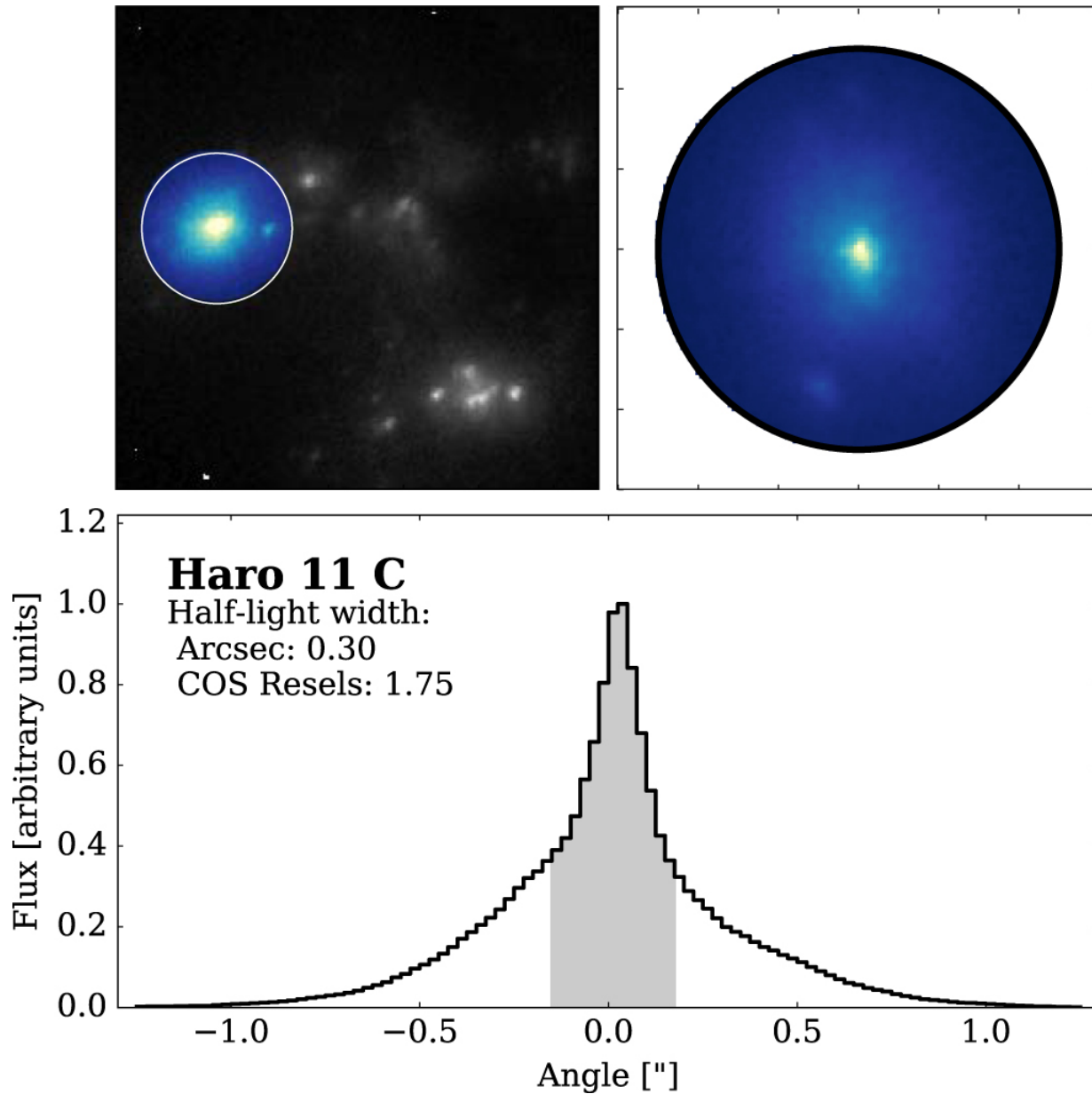
Figure 3. from Neutral ISM, Ly, and Lyman-continuum in the Nearby Starburst Haro 11 null 2017 APJ 837 29 doi:10.3847/1538-4357/aa5d0a https://dx.doi.org/10.3847/1538-4357/aa5d0a © 2017. The American Astronomical Society. All rights reserved.
