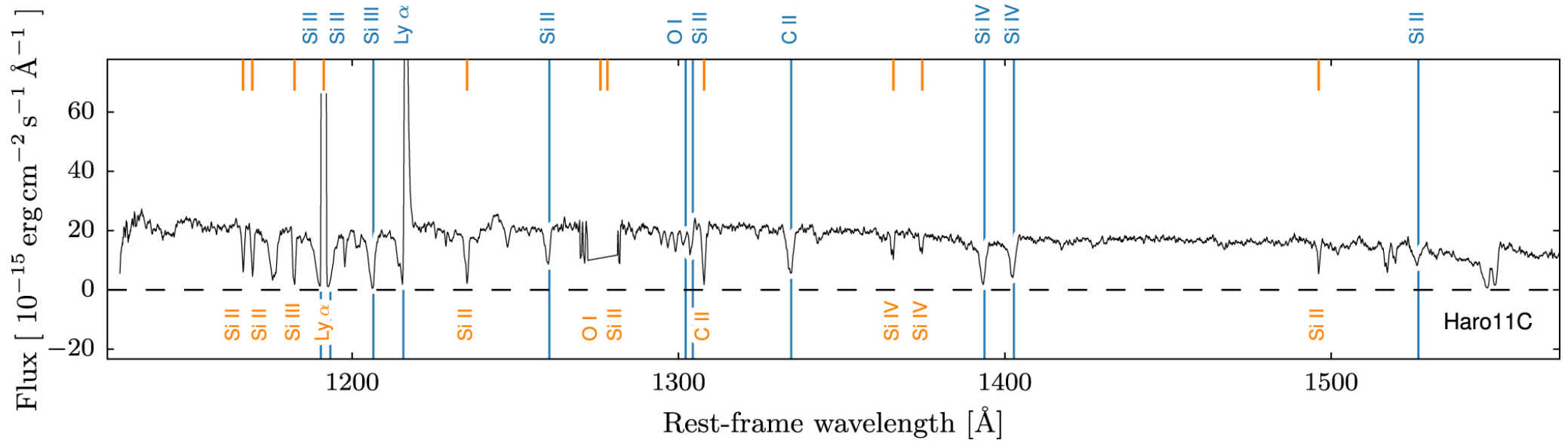
Figure 2. from Neutral ISM, Ly, and Lyman-continuum in the Nearby Starburst Haro 11 null 2017 APJ 837 29 doi:10.3847/1538-4357/aa5d0a https://dx.doi.org/10.3847/1538-4357/aa5d0a © 2017. The American Astronomical Society. All rights reserved.
