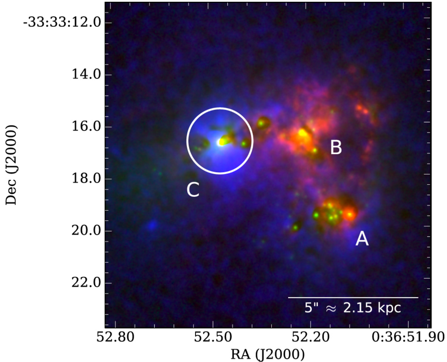
Figure 1. from Neutral ISM, Ly, and Lyman-continuum in the Nearby Starburst Haro 11 null 2017 APJ 837 29 doi:10.3847/1538-4357/aa5d0a https://dx.doi.org/10.3847/1538-4357/aa5d0a © 2017. The American Astronomical Society. All rights reserved.
