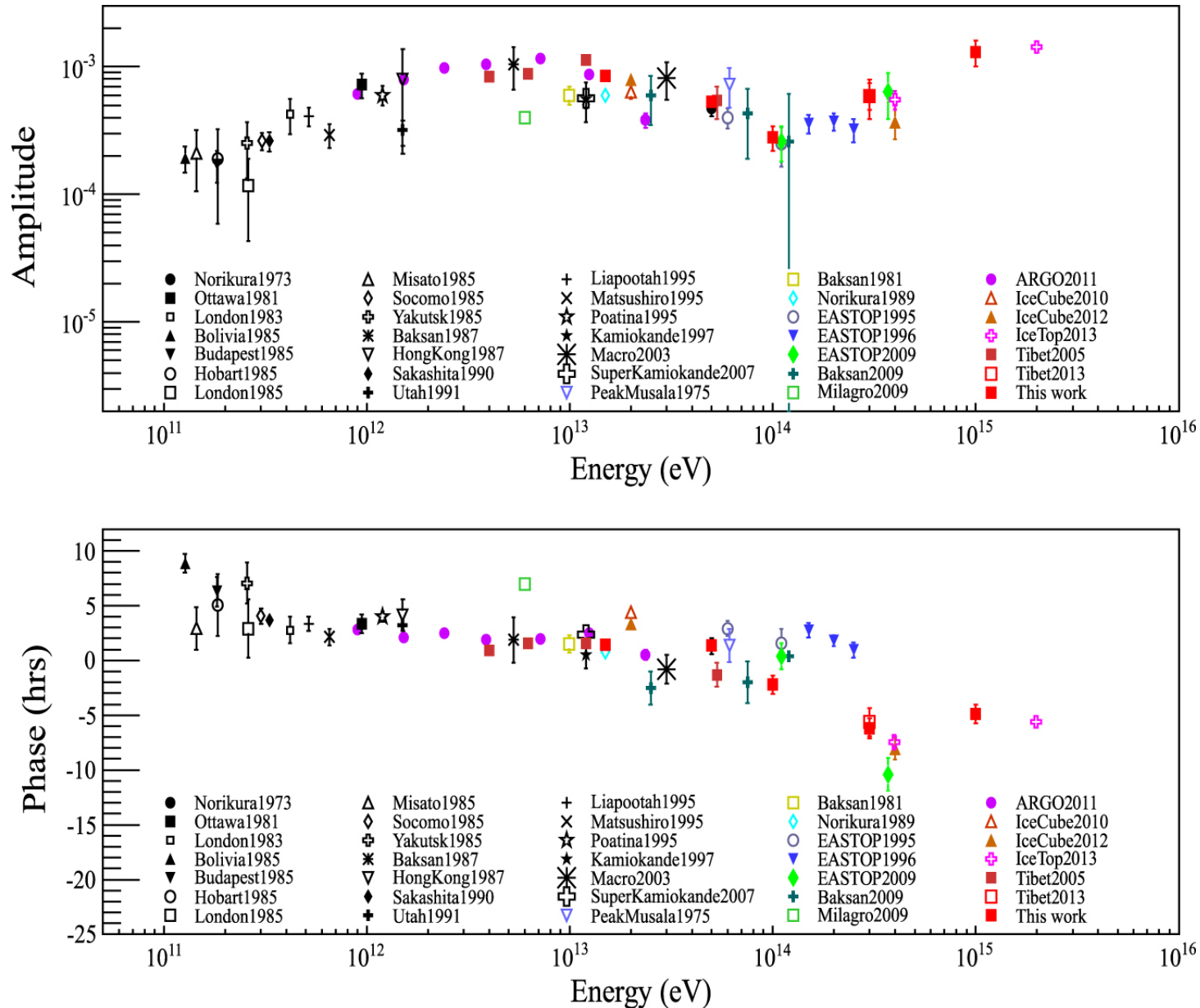
Figure 5. from Northern Sky Galactic Cosmic Ray Anisotropy between 10 and 1000 TeV with the Tibet Air Shower Array null 2017 APJ 836 153 doi:10.3847/1538-4357/836/2/153 https://dx.doi.org/10.3847/1538-4357/836/2/153 © 2017. The American Astronomical Society. All rights reserved.
