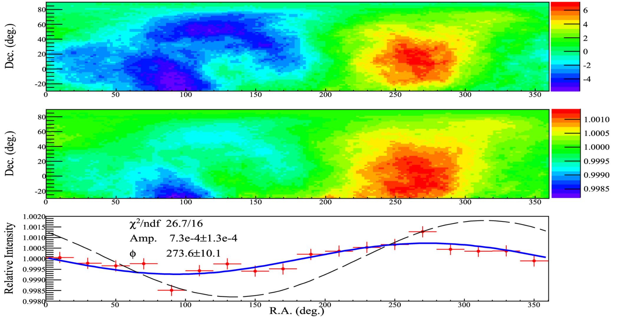
Figure 3. from Northern Sky Galactic Cosmic Ray Anisotropy between 10 and 1000 TeV with the Tibet Air Shower Array null 2017 APJ 836 153 doi:10.3847/1538-4357/836/2/153 https://dx.doi.org/10.3847/1538-4357/836/2/153 © 2017. The American Astronomical Society. All rights reserved.
