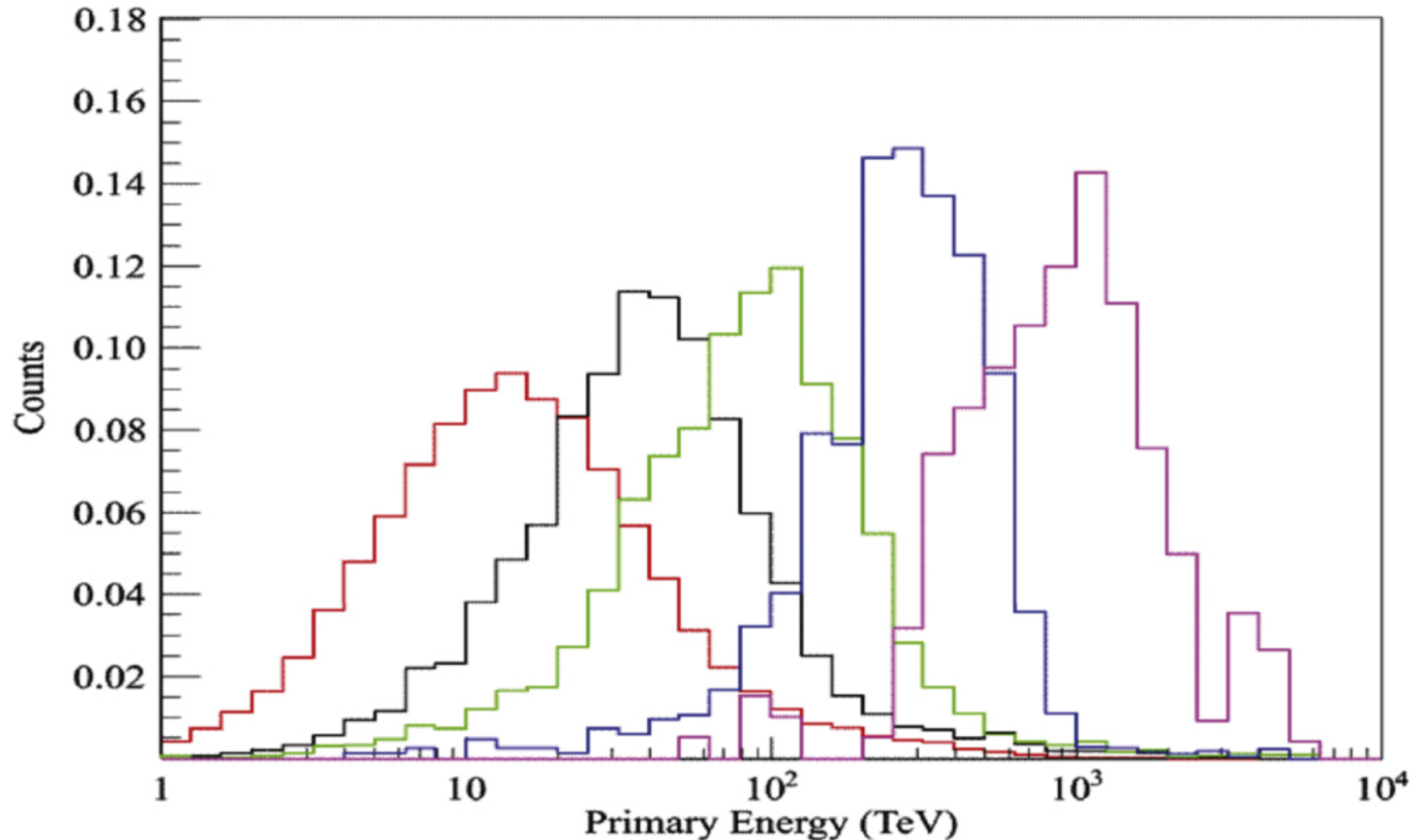
Figure 2. from Northern Sky Galactic Cosmic Ray Anisotropy between 10 and 1000 TeV with the Tibet Air Shower Array null 2017 APJ 836 153 doi:10.3847/1538-4357/836/2/153 https://dx.doi.org/10.3847/1538-4357/836/2/153 © 2017. The American Astronomical Society. All rights reserved.
