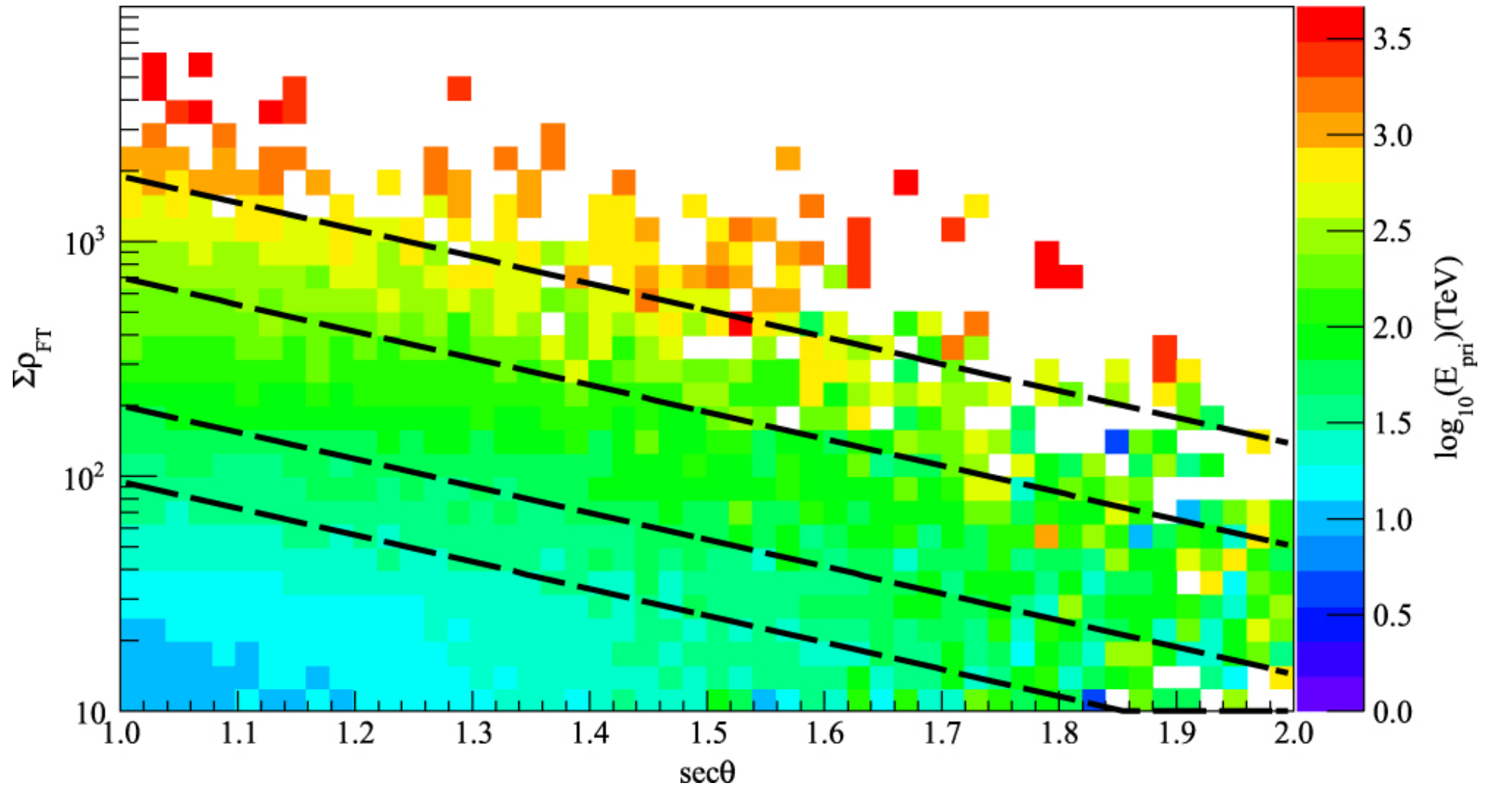
Figure 1. from Northern Sky Galactic Cosmic Ray Anisotropy between 10 and 1000 TeV with the Tibet Air Shower Array null 2017 APJ 836 153 doi:10.3847/1538-4357/836/2/153 https://dx.doi.org/10.3847/1538-4357/836/2/153 © 2017. The American Astronomical Society. All rights reserved.
