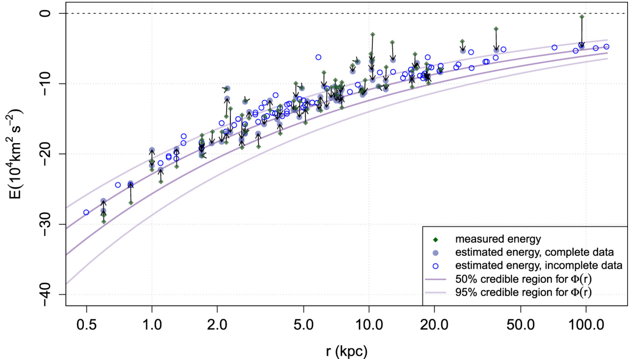
Figure 8. from Bayesian Mass Estimates of the Milky Way: Including Measurement Uncertainties with Hierarchical Bayes null 2017 APJ 835 167 doi:10.3847/1538-4357/835/2/167 https://dx.doi.org/10.3847/1538-4357/835/2/167 © 2017. The American Astronomical Society. All rights reserved.
