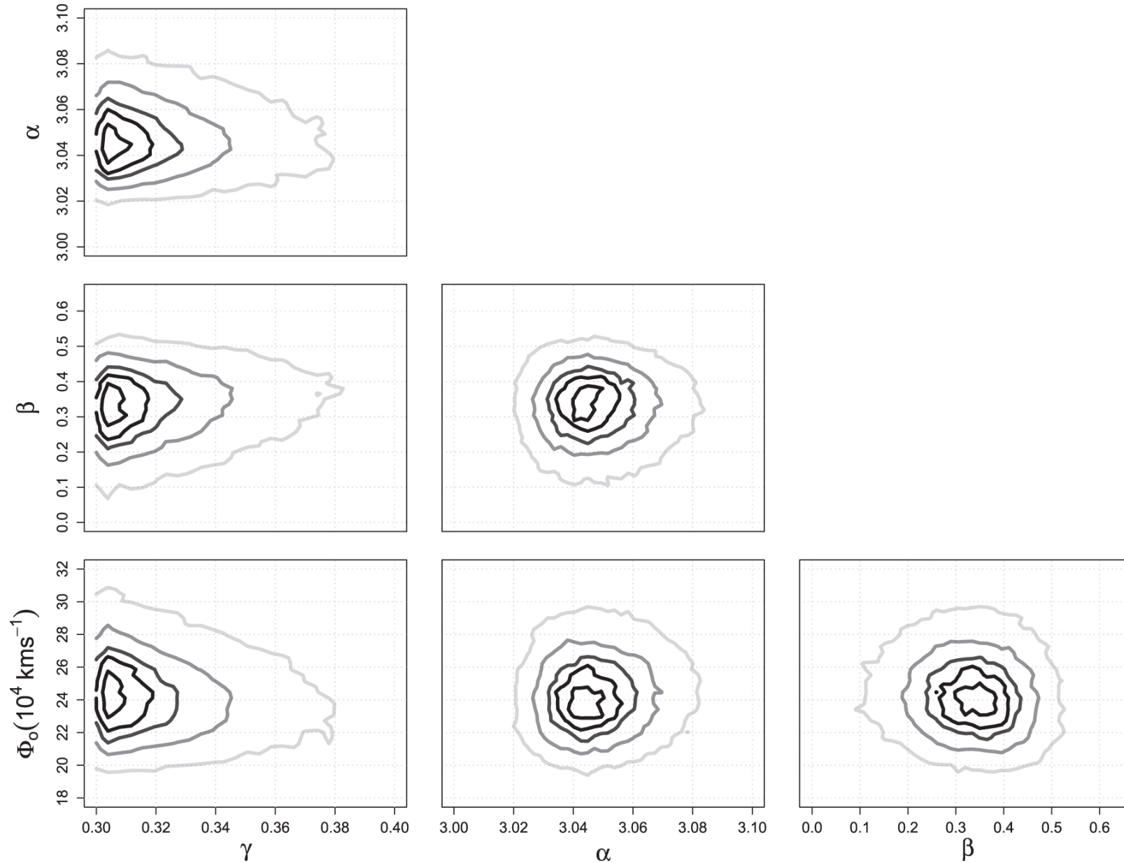
Figure 7. from Bayesian Mass Estimates of the Milky Way: Including Measurement Uncertainties with Hierarchical Bayes null 2017 APJ 835 167 doi:10.3847/1538-4357/835/2/167 https://dx.doi.org/10.3847/1538-4357/835/2/167 © 2017. The American Astronomical Society. All rights reserved.
