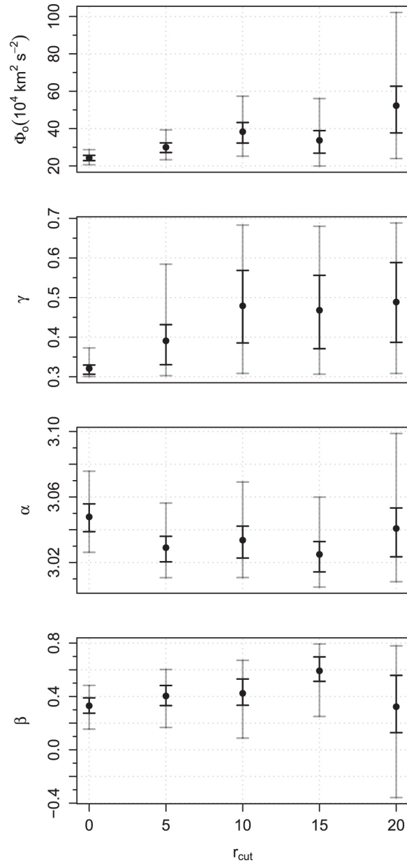
Figure 6. from Bayesian Mass Estimates of the Milky Way: Including Measurement Uncertainties with Hierarchical Bayes null 2017 APJ 835 167 doi:10.3847/1538-4357/835/2/167 https://dx.doi.org/10.3847/1538-4357/835/2/167 © 2017. The American Astronomical Society. All rights reserved.
