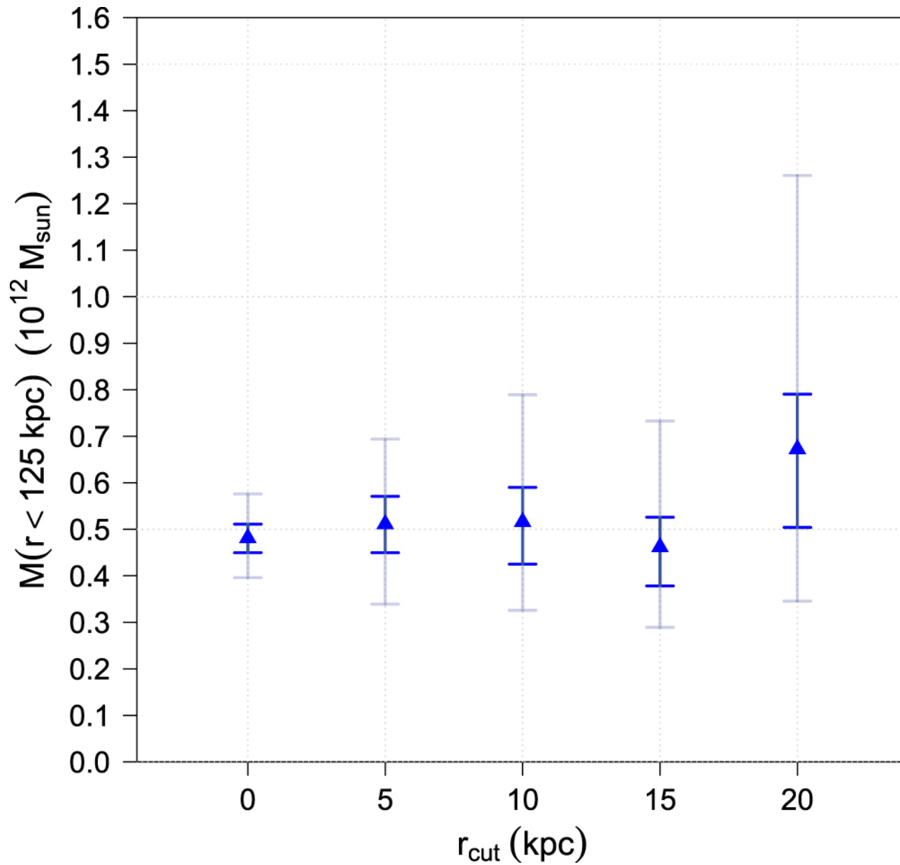
Figure 5. from Bayesian Mass Estimates of the Milky Way: Including Measurement Uncertainties with Hierarchical Bayes null 2017 APJ 835 167 doi:10.3847/1538-4357/835/2/167 https://dx.doi.org/10.3847/1538-4357/835/2/167 © 2017. The American Astronomical Society. All rights reserved.
