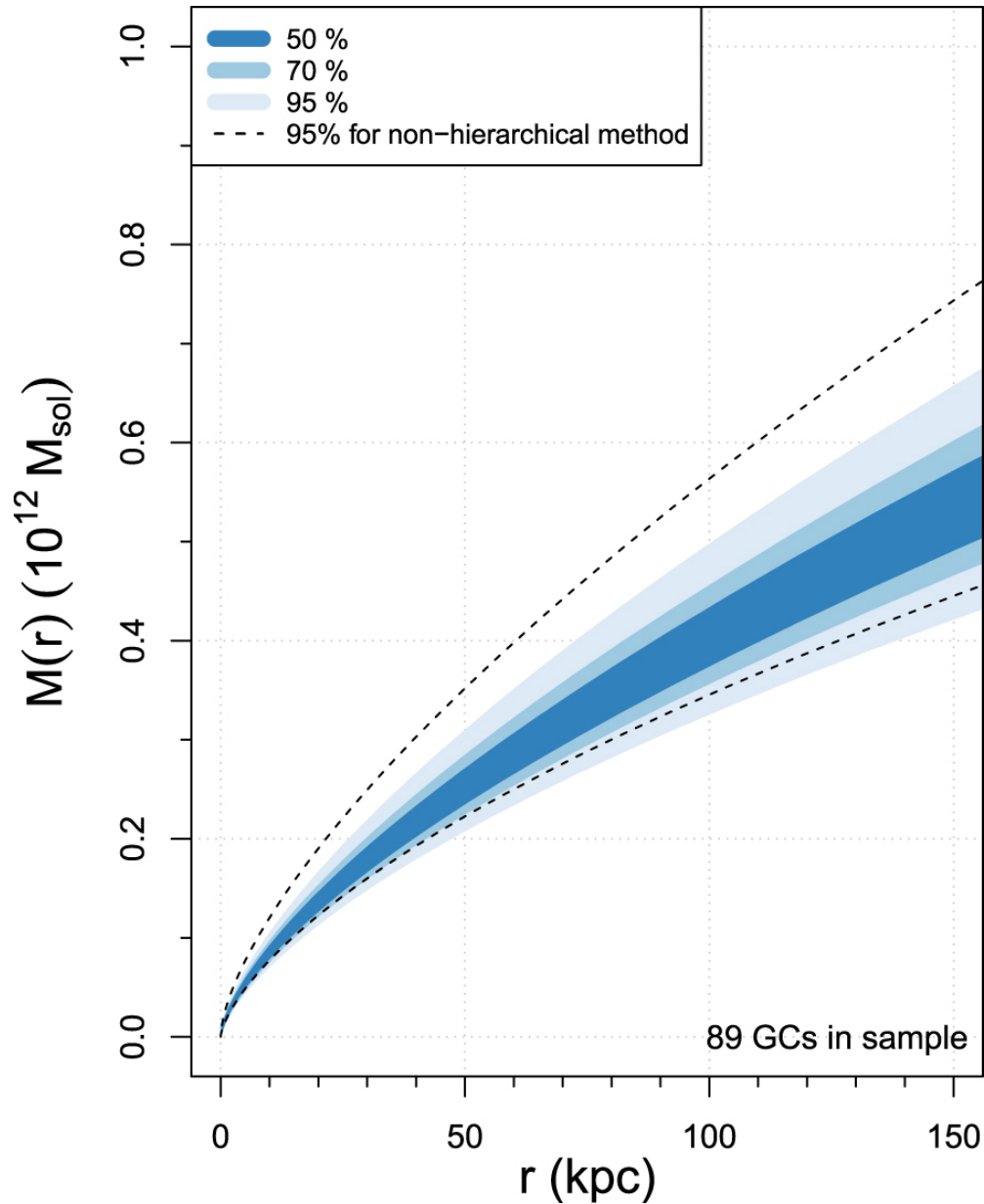
Figure 3. from Bayesian Mass Estimates of the Milky Way: Including Measurement Uncertainties with Hierarchical Bayes null 2017 APJ 835 167 doi:10.3847/1538-4357/835/2/167 https://dx.doi.org/10.3847/1538-4357/835/2/167 © 2017. The American Astronomical Society. All rights reserved.
