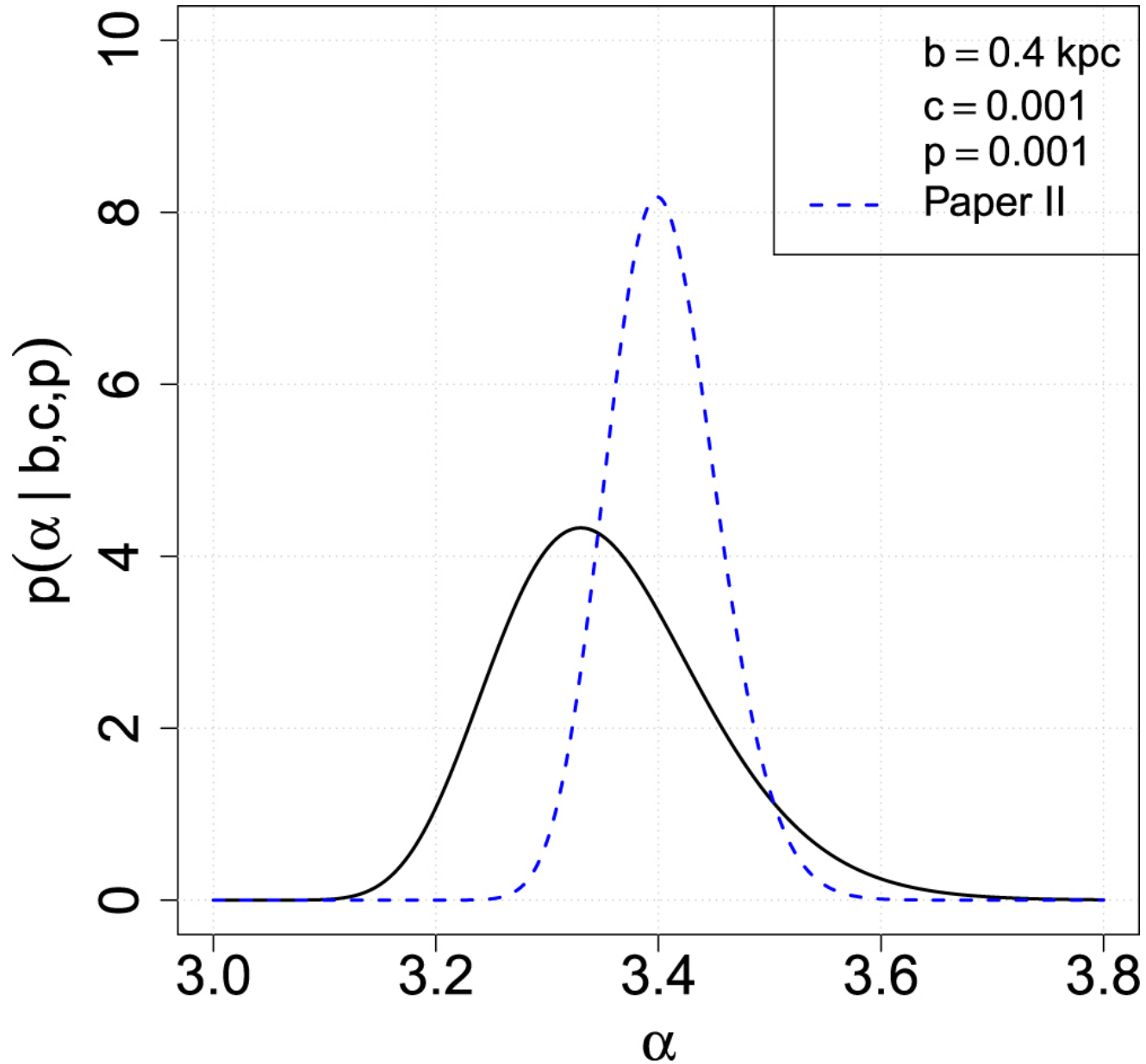
Figure 1. from Bayesian Mass Estimates of the Milky Way: Including Measurement Uncertainties with Hierarchical Bayes null 2017 APJ 835 167 doi:10.3847/1538-4357/835/2/167 https://dx.doi.org/10.3847/1538-4357/835/2/167 © 2017. The American Astronomical Society. All rights reserved.
