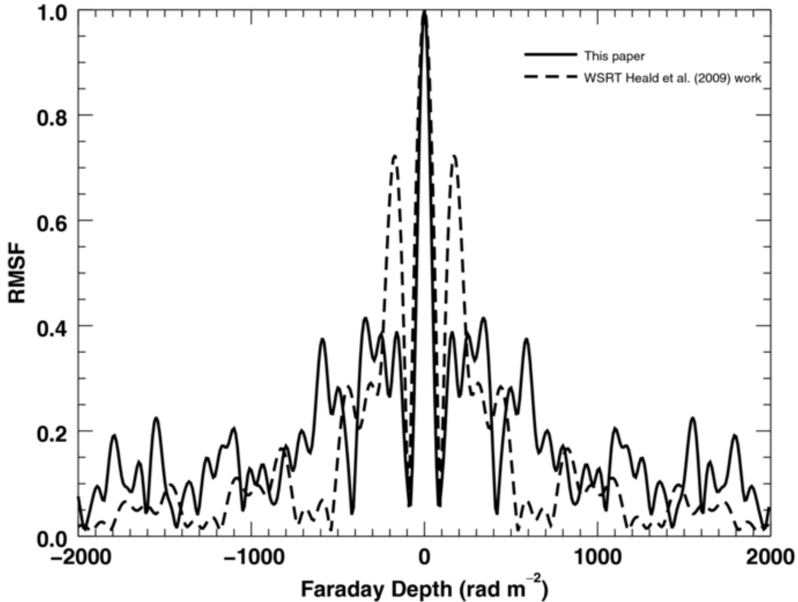
Figure 3. from Properties of the Magneto-ionic Medium in the Halo of M51 Revealed by Wide-band Polarimetry Mao et al. 2015 ApJ 800 92 doi:10.1088/0004-637X/800/2/92 http://dx.doi.org/10.1088/0004-637X/800/2/92 © 2015. The American Astronomical Society. All rights reserved.
