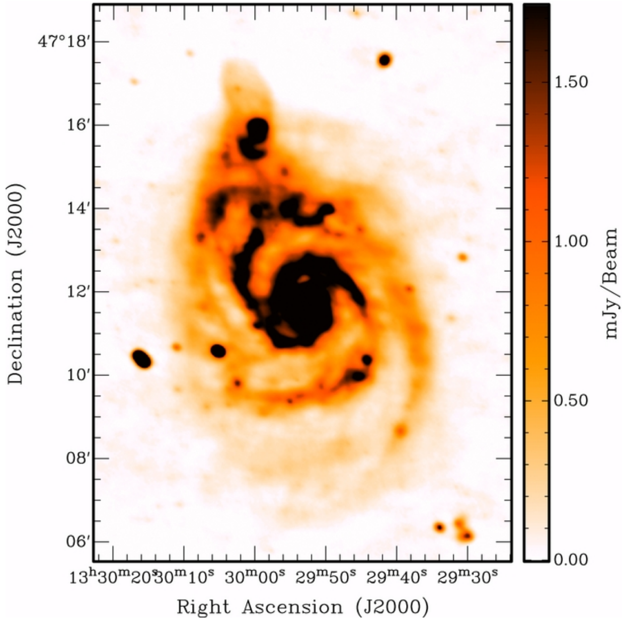
Figure 1. from Properties of the Magneto-ionic Medium in the Halo of M51 Revealed by Wide-band Polarimetry Mao et al. 2015 ApJ 800 92 doi:10.1088/0004-637X/800/2/92 http://dx.doi.org/10.1088/0004-637X/800/2/92 © 2015. The American Astronomical Society. All rights reserved.
