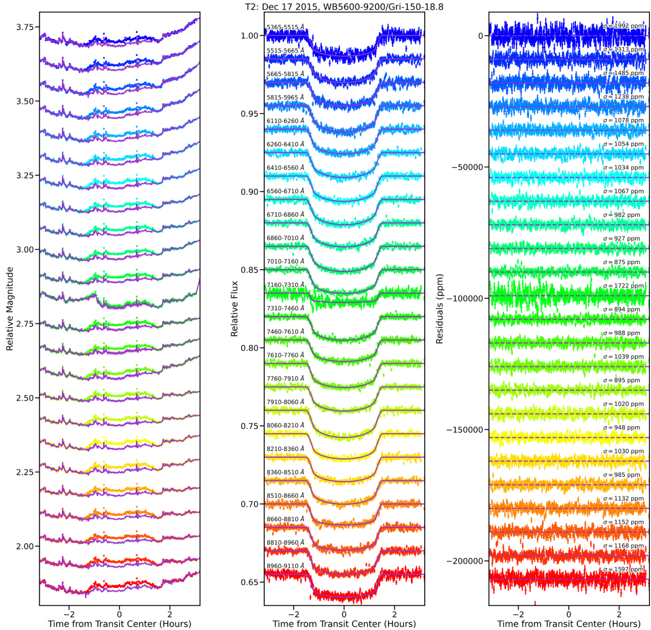
Figure 9. from Natalie H. Allen et al 2022 Astron. J. 164 doi:10.3847/1538-3881/ac8b74 https://dx.doi.org/10.3847/1538-3881/ac8b74 © 2022. The Author(s). Published by the American Astronomical Society.
