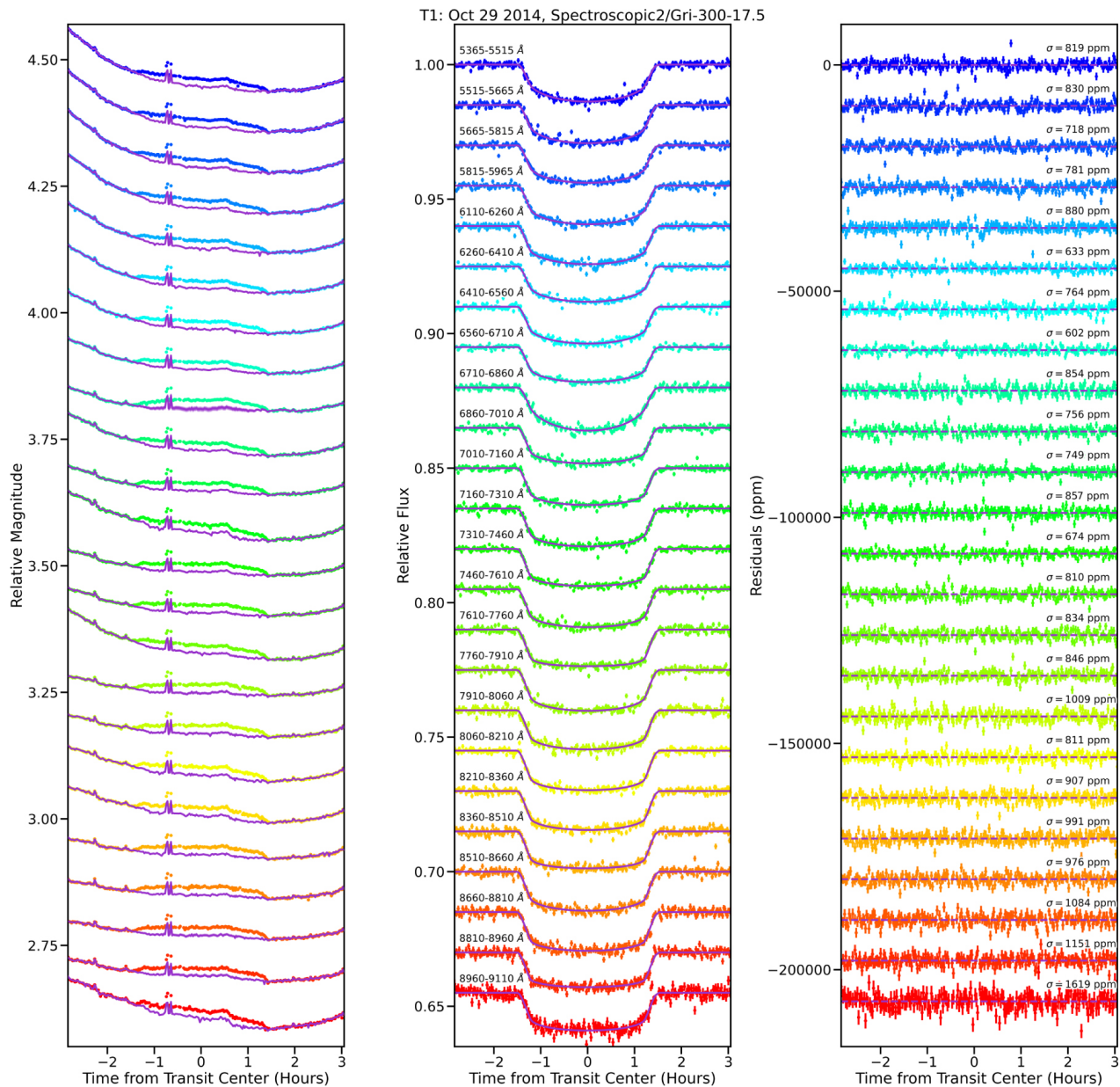
Figure 8. from Natalie H. Allen et al 2022 Astron. J. 164 doi:10.3847/1538-3881/ac8b74 https://dx.doi.org/10.3847/1538-3881/ac8b74 © 2022. The Author(s). Published by the American Astronomical Society.
