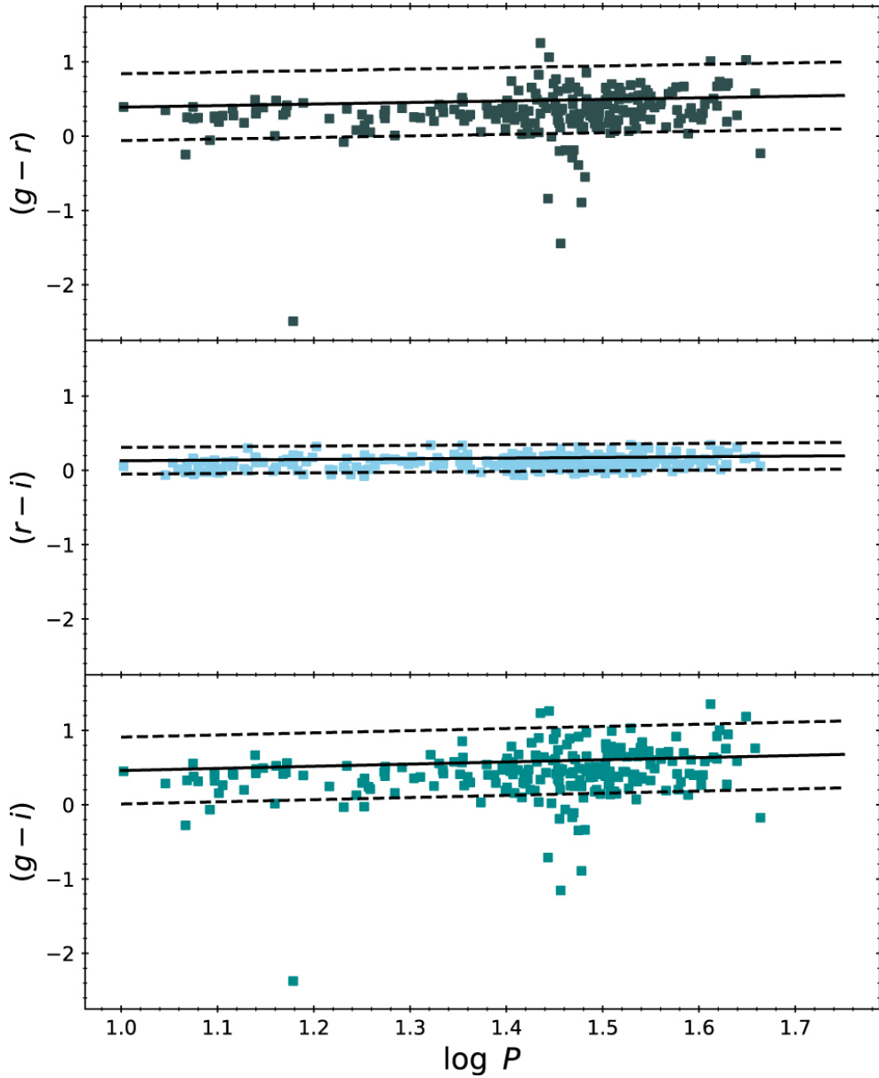
Figure 8. from Chow-Choong Ngeow et al 2022 Astron. J. 164 doi:10.3847/1538-3881/ac87a4 http://dx.doi.org/10.3847/1538-3881/ac87a4 © 2022. The Author(s). Published by the American Astronomical Society.
