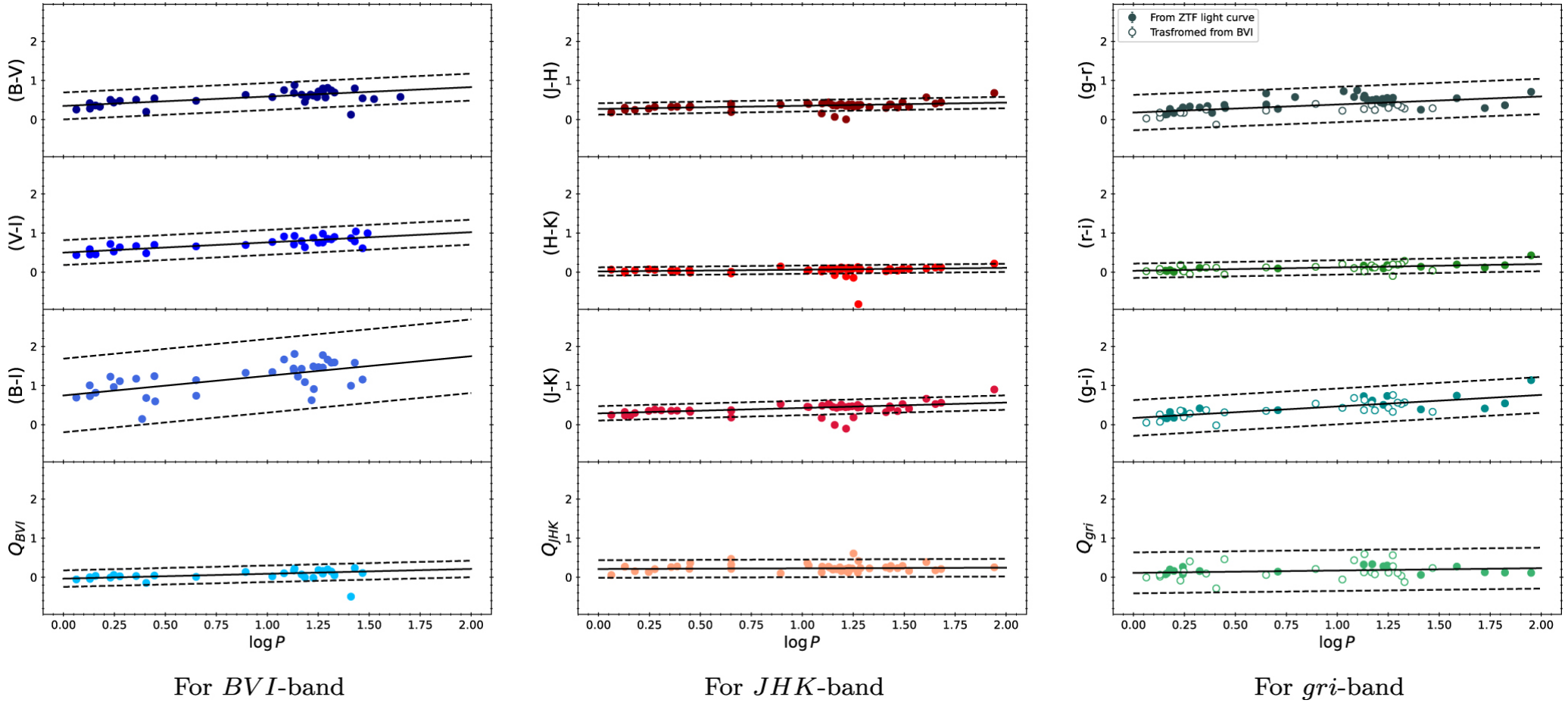
Figure 7. from Chow-Choong Ngeow et al 2022 Astron. J. 164 doi:10.3847/1538-3881/ac87a4 http://dx.doi.org/10.3847/1538-3881/ac87a4 © 2022. The Author(s). Published by the American Astronomical Society.
