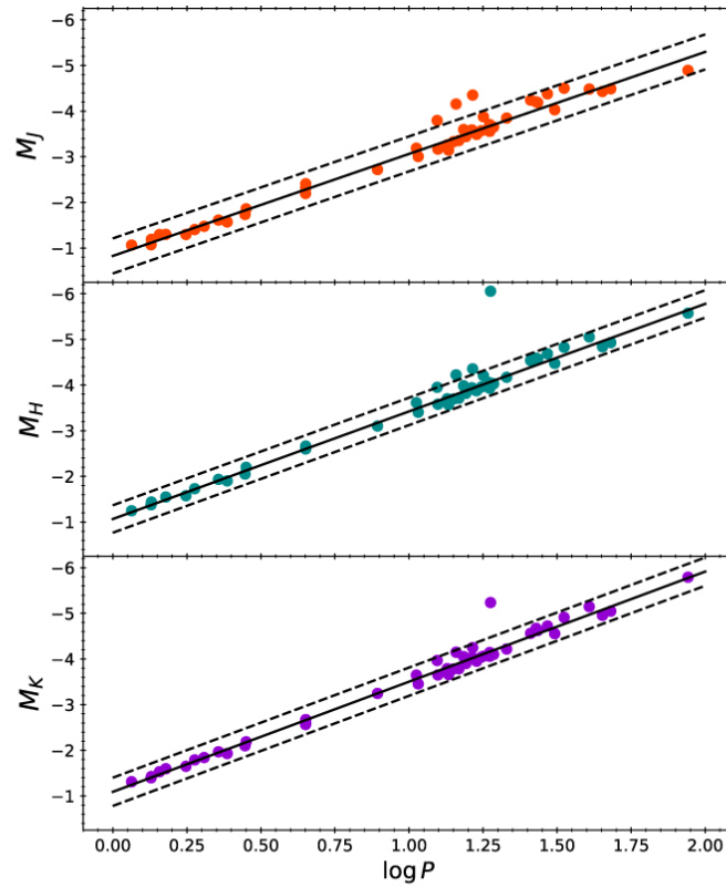
JHK -band PL relations
