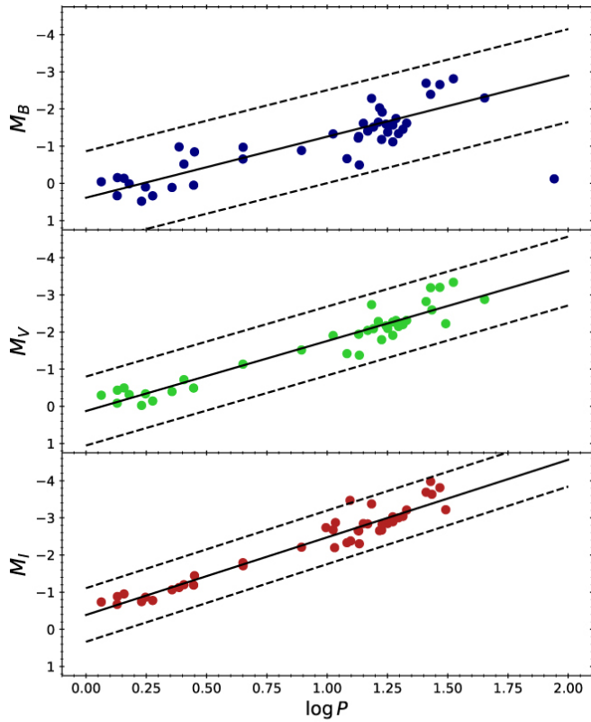
BVI -band PL relations
