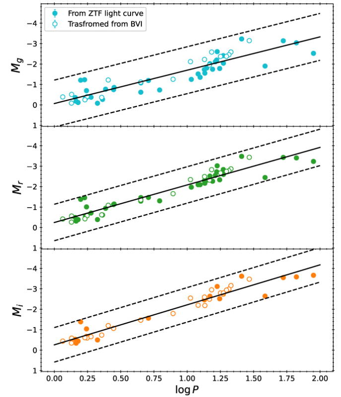
gri -band PL relations
