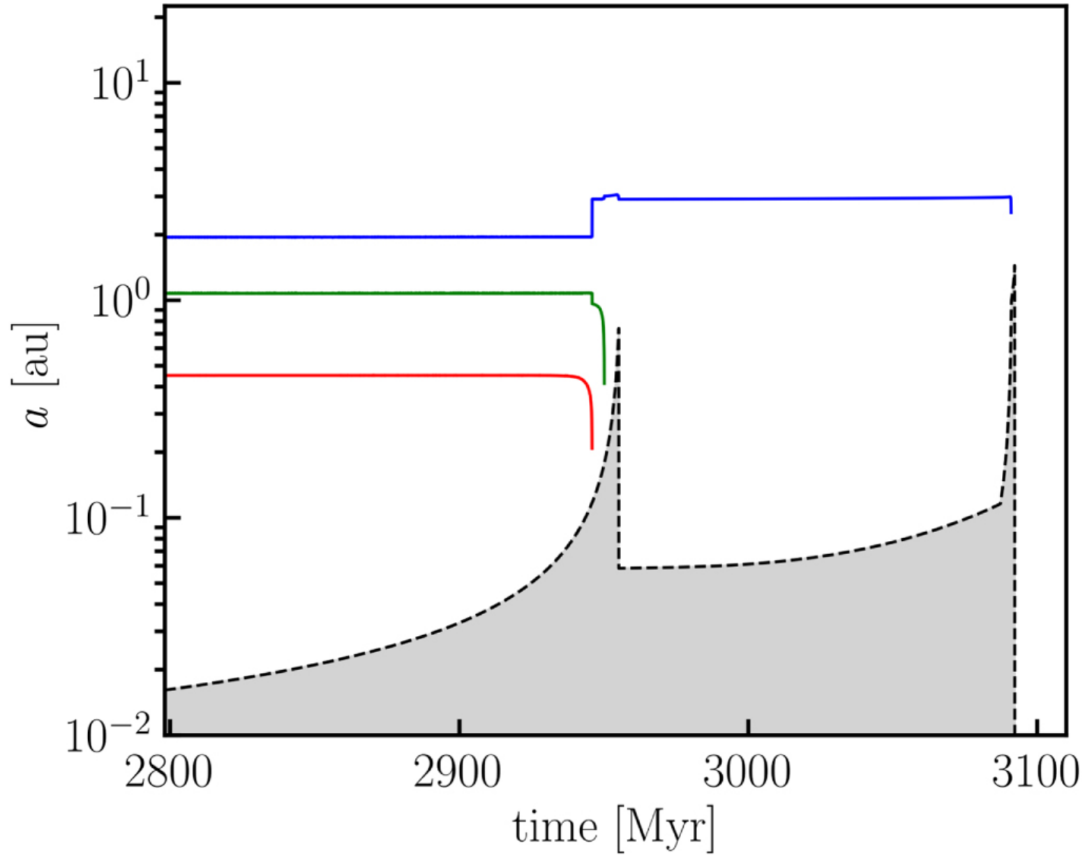
Figure 7. from Trifon Trifonov et al 2022 Astron. J. 164 doi:10.3847/1538-3881/ac7ce0 http://dx.doi.org/10.3847/1538-3881/ac7ce0 © 2022. The Author(s). Published by the American Astronomical Society.
