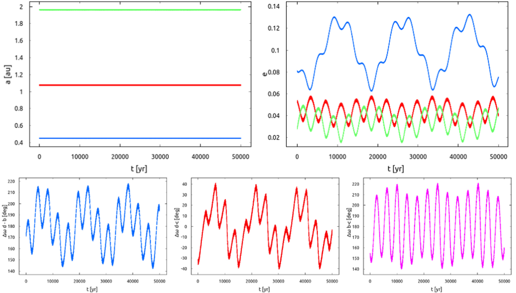
Figure 5. from Trifon Trifonov et al 2022 Astron. J. 164 doi:10.3847/1538-3881/ac7ce0 http://dx.doi.org/10.3847/1538-3881/ac7ce0 © 2022. The Author(s). Published by the American Astronomical Society.
