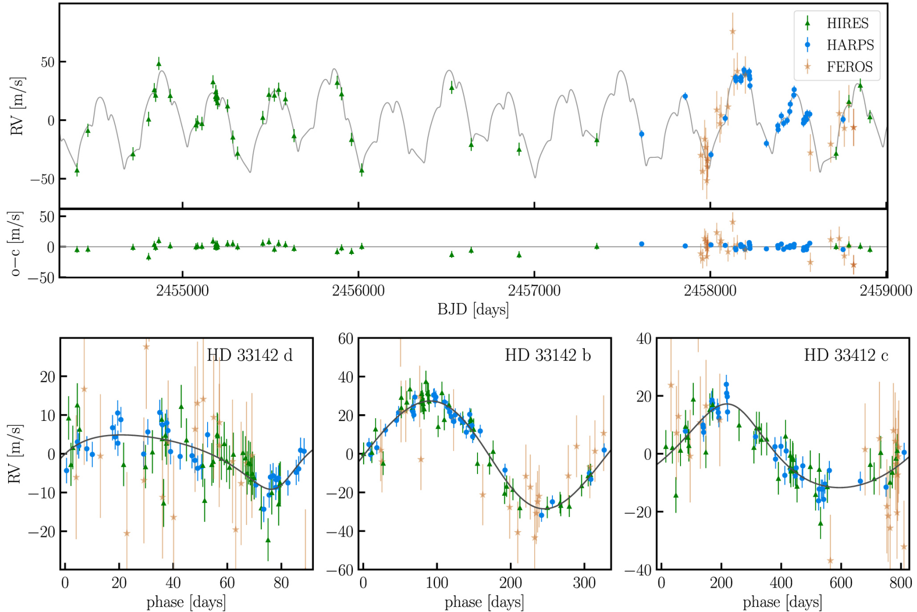
Figure 3. from Trifon Trifonov et al 2022 Astron. J. 164 doi:10.3847/1538-3881/ac7ce0 http://dx.doi.org/10.3847/1538-3881/ac7ce0 © 2022. The Author(s). Published by the American Astronomical Society.
