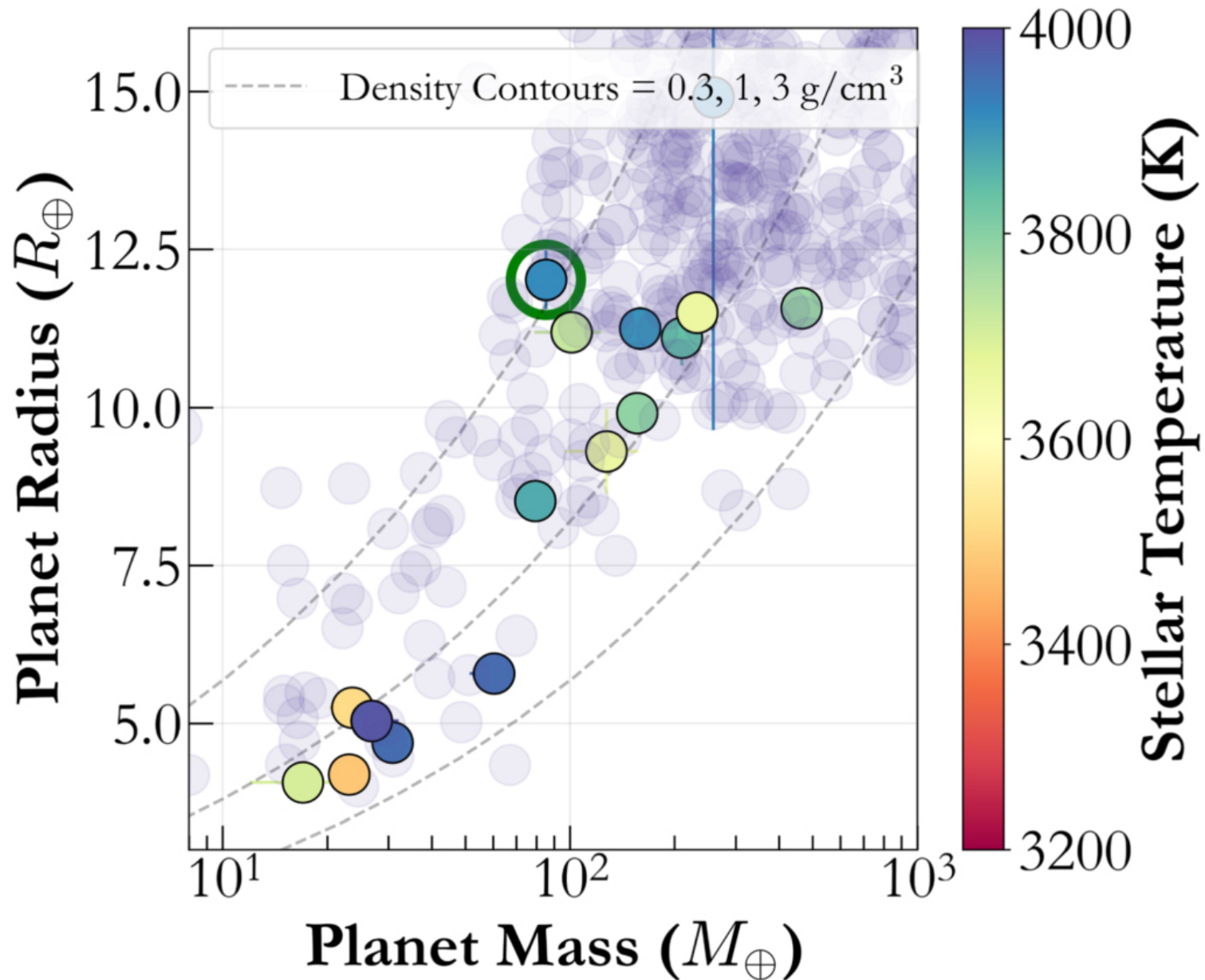
Figure 9. from Shubham Kanodia et al 2022 Astron. J. 164 doi:10.3847/1538-3881/ac7c20 https://dx.doi.org/10.3847/1538-3881/ac7c20 © 2022. The Author(s). Published by the American Astronomical Society.
