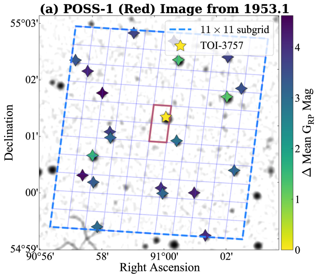
Figure 5. from Shubham Kanodia et al 2022 Astron. J. 164 doi:10.3847/1538-3881/ac7c20 https://dx.doi.org/10.3847/1538-3881/ac7c20 © 2022. The Author(s). Published by the American Astronomical Society.
