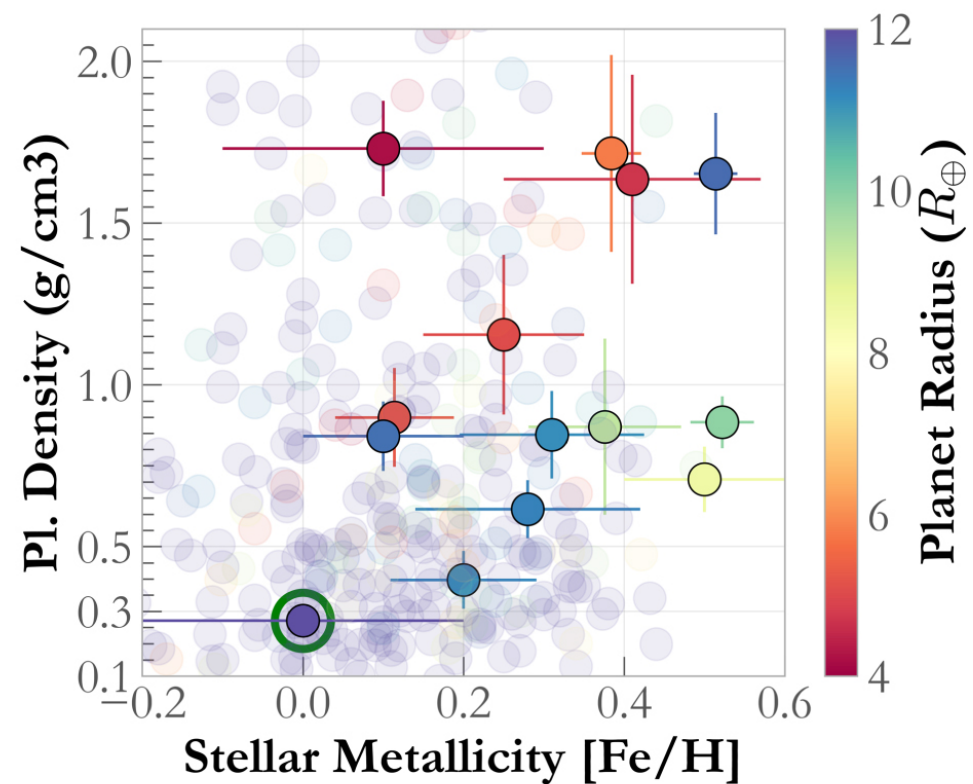
b) Planet density as a function of stellar metallicity
