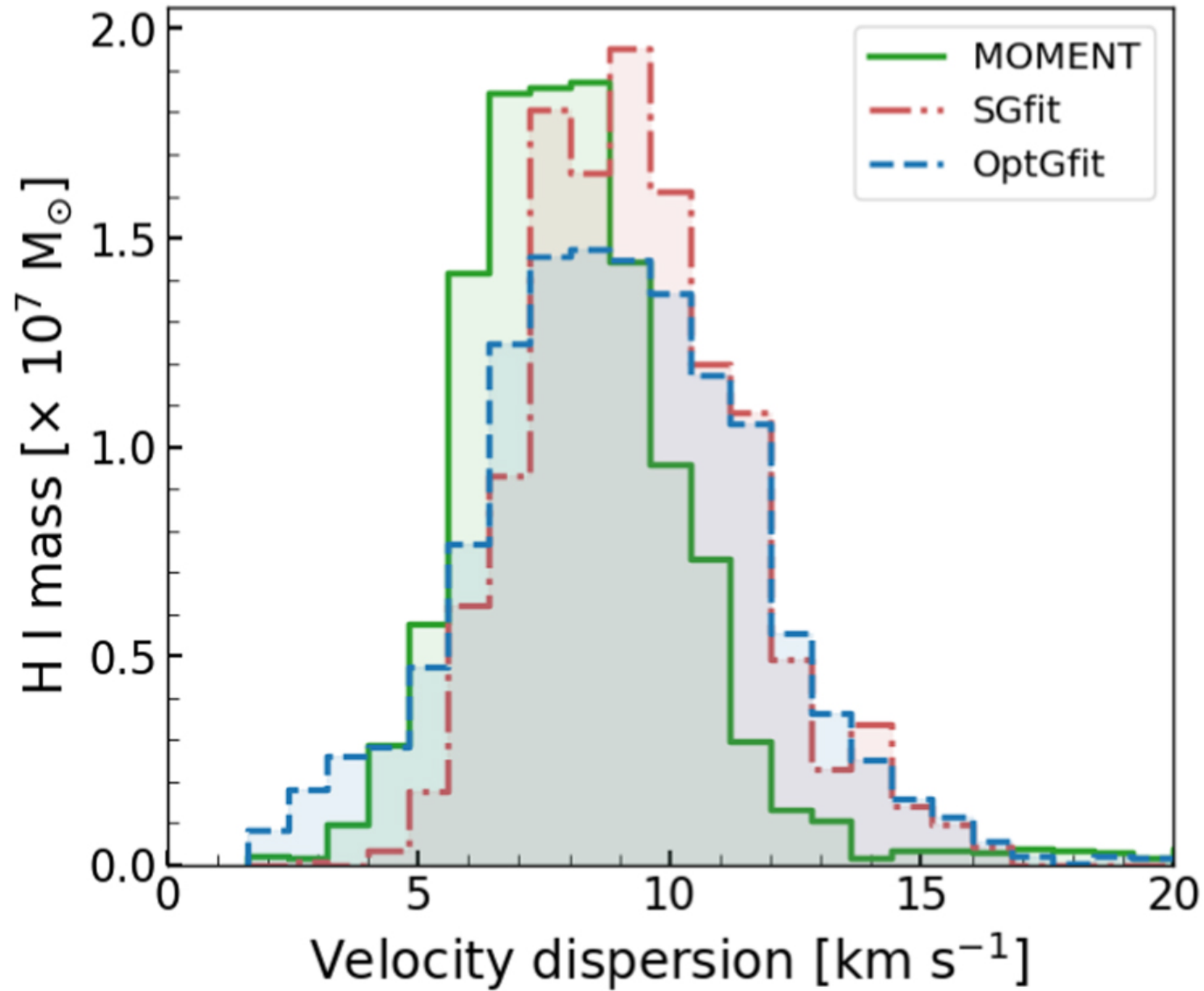
Figure 6. from Hye-Jin Park et al 2022 Astron. J. 164 doi:10.3847/1538-3881/ac7c1b https://dx.doi.org/10.3847/1538-3881/ac7c1b © 2022. The Author(s). Published by the American Astronomical Society.
