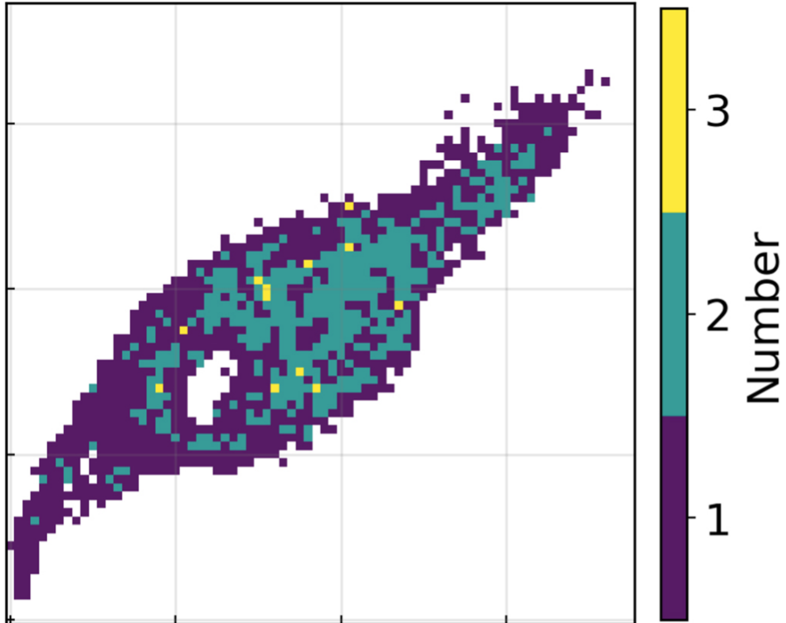
Figure 5. from Hye-Jin Park et al 2022 Astron. J. 164 doi:10.3847/1538-3881/ac7c1b http://dx.doi.org/10.3847/1538-3881/ac7c1b © 2022. The Author(s). Published by the American Astronomical Society.
