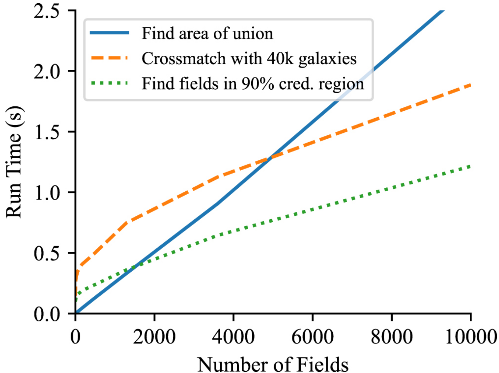
Figure 5. from Leo P. Singer et al 2022 Astron. J. 163 doi:10.3847/1538-3881/ac5ab8 https://dx.doi.org/10.3847/1538-3881/ac5ab8 © 2022. The Author(s). Published by the American Astronomical Society.
